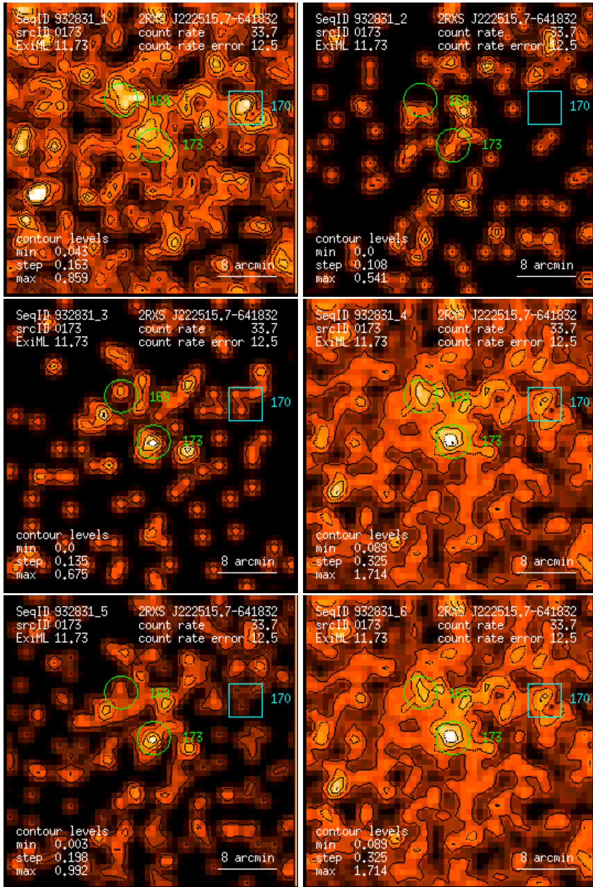
Figure 173: RASS 932831: detection 0173: band rate images, Gaussian filter: (1) PSPC channels 11 – 41, (2) 52 – 90, (3) 91 – 201, (4) 11 – 235, (5) 52 – 201, (6) 11 – 201. Broad band rates in counts/ks. Band rate contour levels in counts/ks/arcmin 2 .
