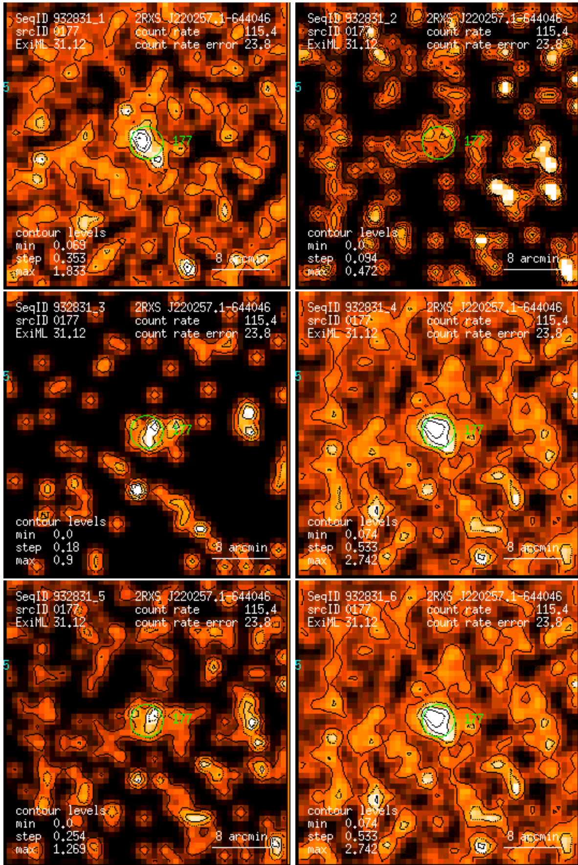
Figure 177: RASS 932831: detection 0177: band rate images, Gaussian filter: (1) PSPC channels 11 – 41, (2) 52 – 90, (3) 91 – 201, (4) 11 – 235, (5) 52 – 201, (6) 11 – 201. Broad band rates in counts/ks. Band rate contour levels in counts/ks/arcmin 2 .
