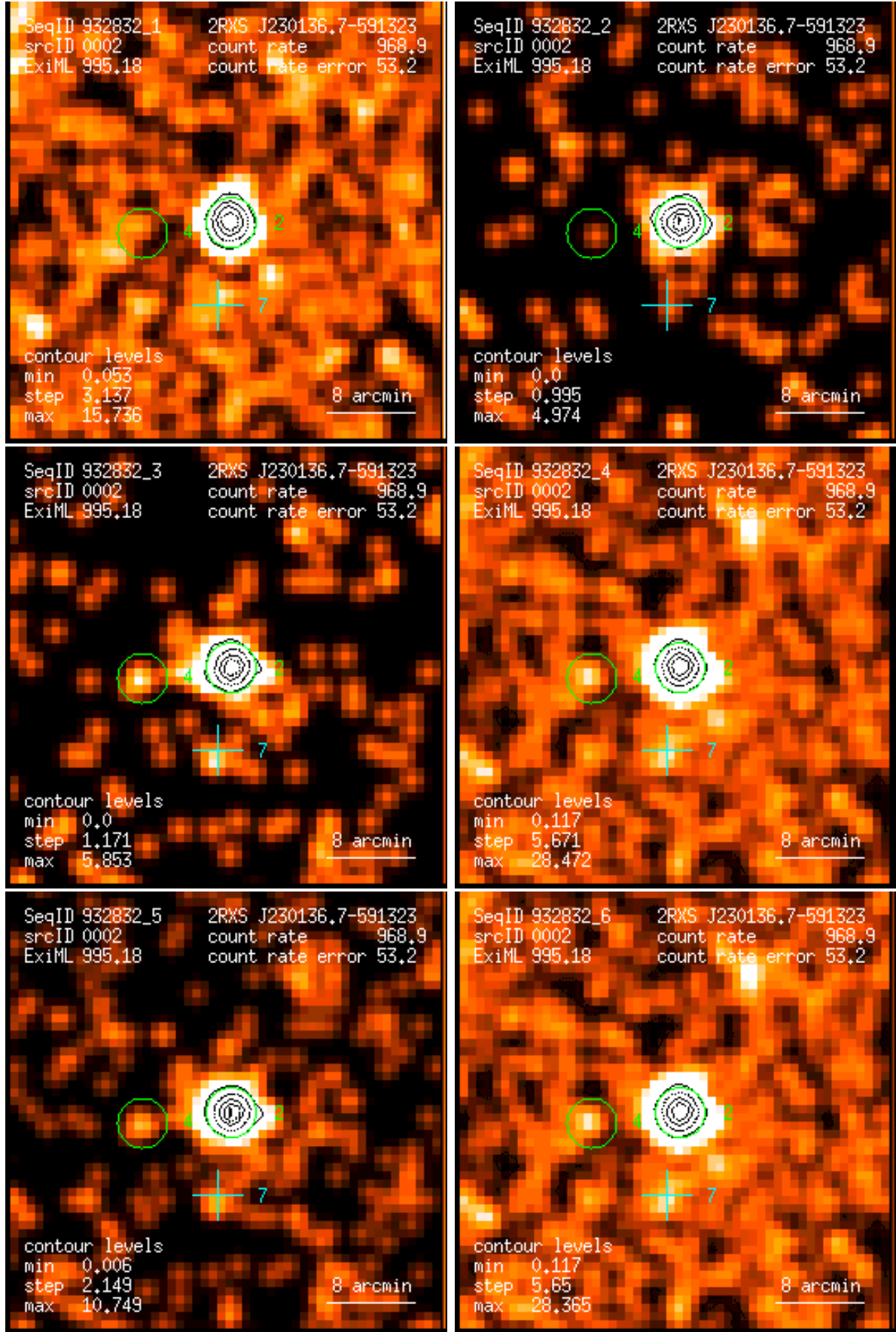
Figure 2: RASS 932832: detection 0002: band rate images, Gaussian filter: (1) PSPC channels 11 – 41, (2) 52 – 90, (3) 91 – 201, (4) 11 – 235, (5) 52 – 201, (6) 11 – 201. Broad band rates in counts/ks. Band rate contour levels in counts/ks/arcmin 2 .
