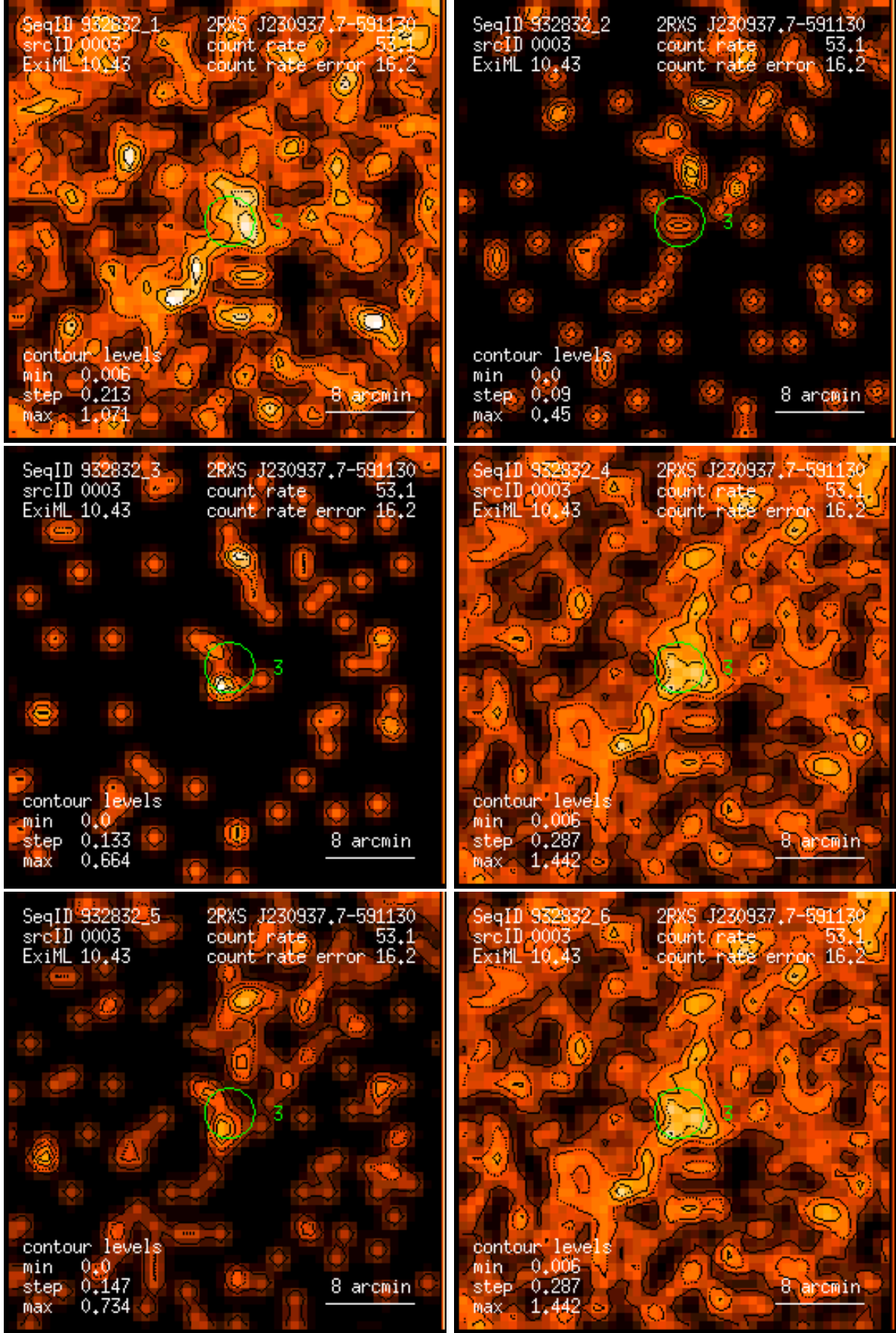
Figure 3: RASS 932832: detection 0003: band rate images, Gaussian filter: (1) PSPC channels 11 – 41, (2) 52 – 90, (3) 91 – 201, (4) 11 – 235, (5) 52 – 201, (6) 11 – 201. Broad band rates in counts/ks. Band rate contour levels in counts/ks/arcmin 2 .
