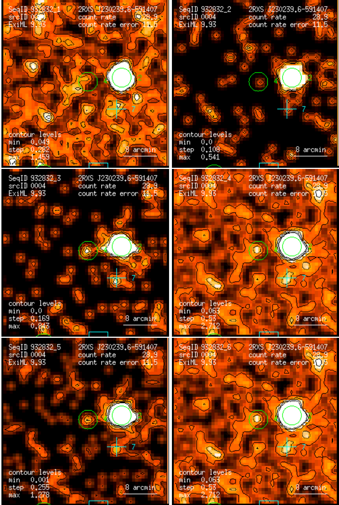
Figure 4: RASS 932832: detection 0004: band rate images, Gaussian filter: (1) PSPC channels 11 – 41, (2) 52 – 90, (3) 91 – 201, (4) 11 – 235, (5) 52 – 201, (6) 11 – 201. Broad band rates in counts/ks. Band rate contour levels in counts/ks/arcmin 2 .
