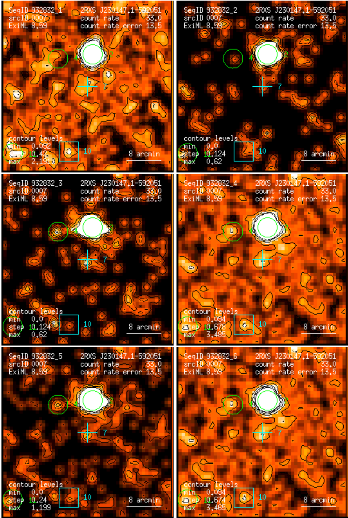
Figure 7: RASS 932832: detection 0007: band rate images, Gaussian filter: (1) PSPC channels 11 – 41, (2) 52 – 90, (3) 91 – 201, (4) 11 – 235, (5) 52 – 201, (6) 11 – 201. Broad band rates in counts/ks. Band rate contour levels in counts/ks/arcmin 2 .
