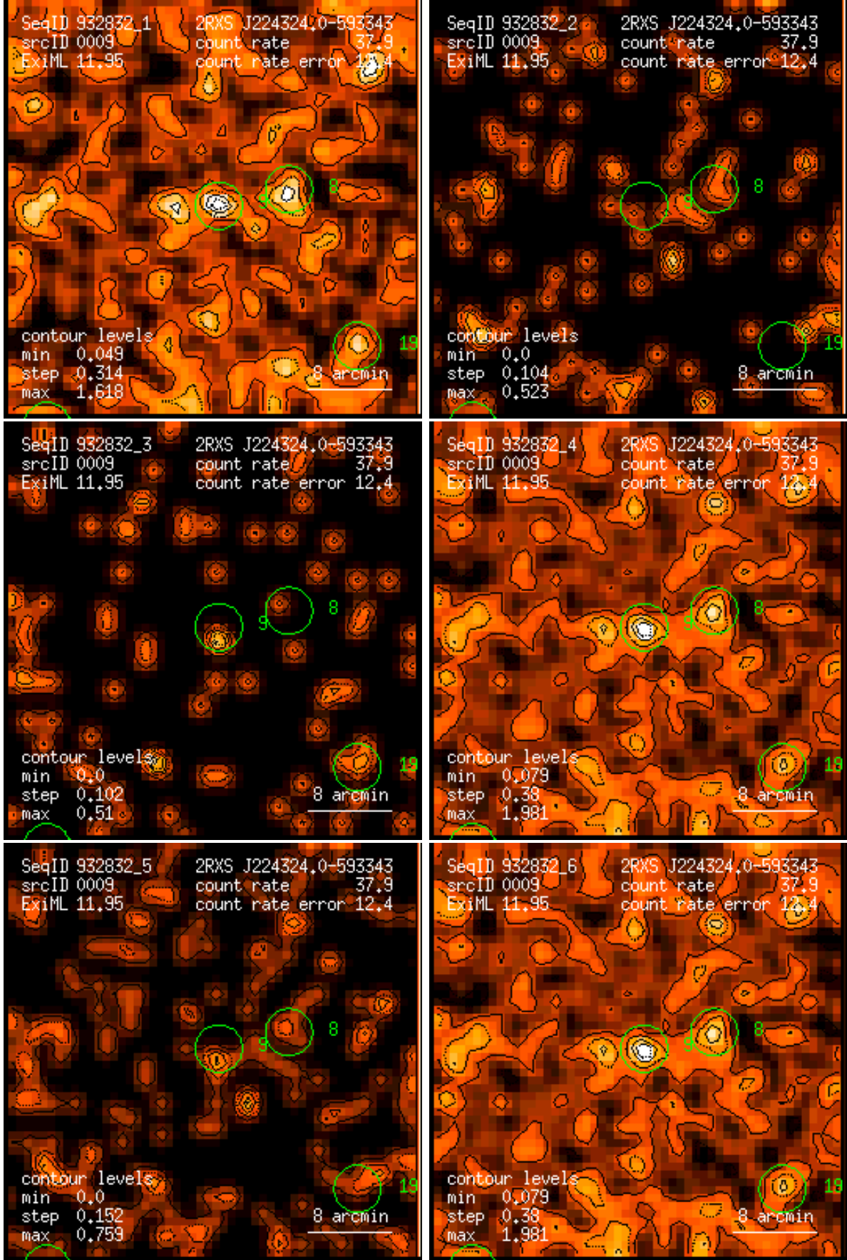
Figure 9: RASS 932832: detection 0009: band rate images, Gaussian filter: (1) PSPC channels 11 – 41, (2) 52 – 90, (3) 91 – 201, (4) 11 – 235, (5) 52 – 201, (6) 11 – 201. Broad band rates in counts/ks. Band rate contour levels in counts/ks/arcmin 2 .
