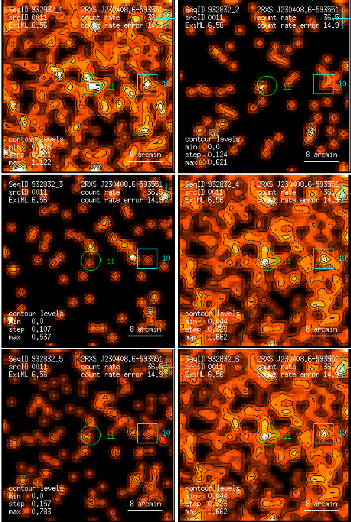
Figure 11: RASS 932832: detection 0011: band rate images, Gaussian filter: (1) PSPC channels 11 – 41, (2) 52 – 90, (3) 91 – 201, (4) 11 – 235, (5) 52 – 201, (6) 11 – 201. Broad band rates in counts/ks. Band rate contour levels in counts/ks/arcmin 2 .
