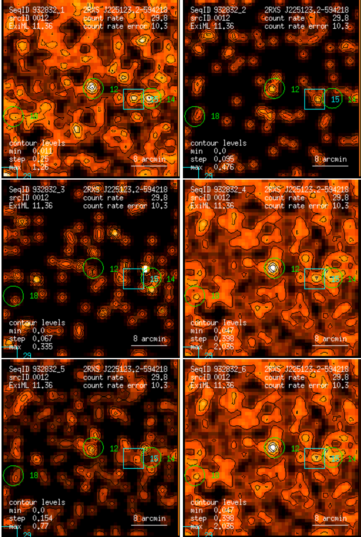
Figure 12: RASS 932832: detection 0012: band rate images, Gaussian filter: (1) PSPC channels 11 – 41, (2) 52 – 90, (3) 91 – 201, (4) 11 – 235, (5) 52 – 201, (6) 11 – 201. Broad band rates in counts/ks. Band rate contour levels in counts/ks/arcmin 2 .
