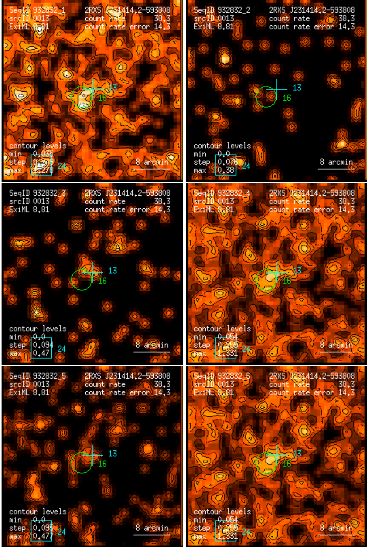
Figure 13: RASS 932832: detection 0013: band rate images, Gaussian filter: (1) PSPC channels 11 – 41, (2) 52 – 90, (3) 91 – 201, (4) 11 – 235, (5) 52 – 201, (6) 11 – 201. Broad band rates in counts/ks. Band rate contour levels in counts/ks/arcmin 2 .
