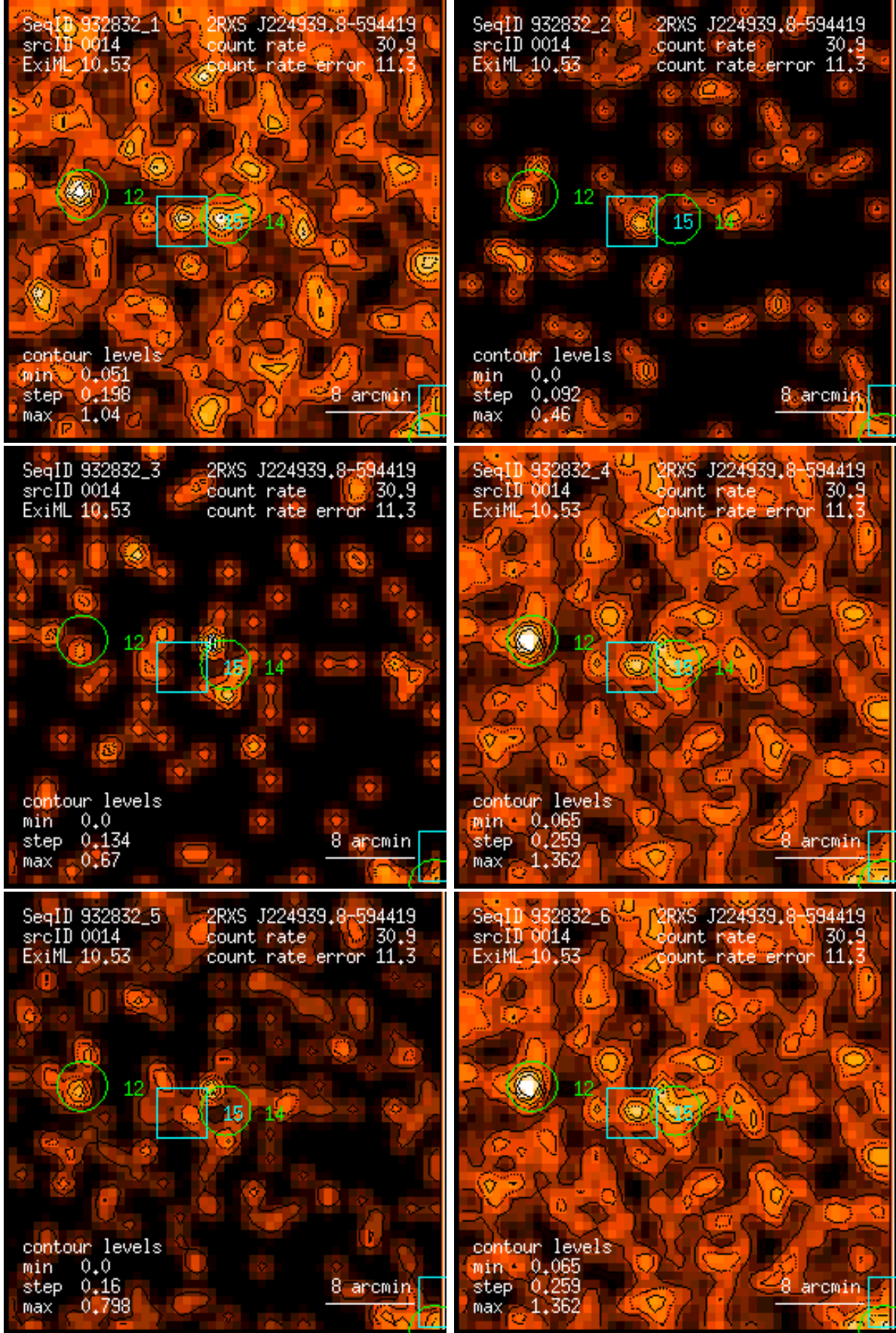
Figure 14: RASS 932832: detection 0014: band rate images, Gaussian filter: (1) PSPC channels 11 – 41, (2) 52 – 90, (3) 91 – 201, (4) 11 – 235, (5) 52 – 201, (6) 11 – 201. Broad band rates in counts/ks. Band rate contour levels in counts/ks/arcmin 2 .
