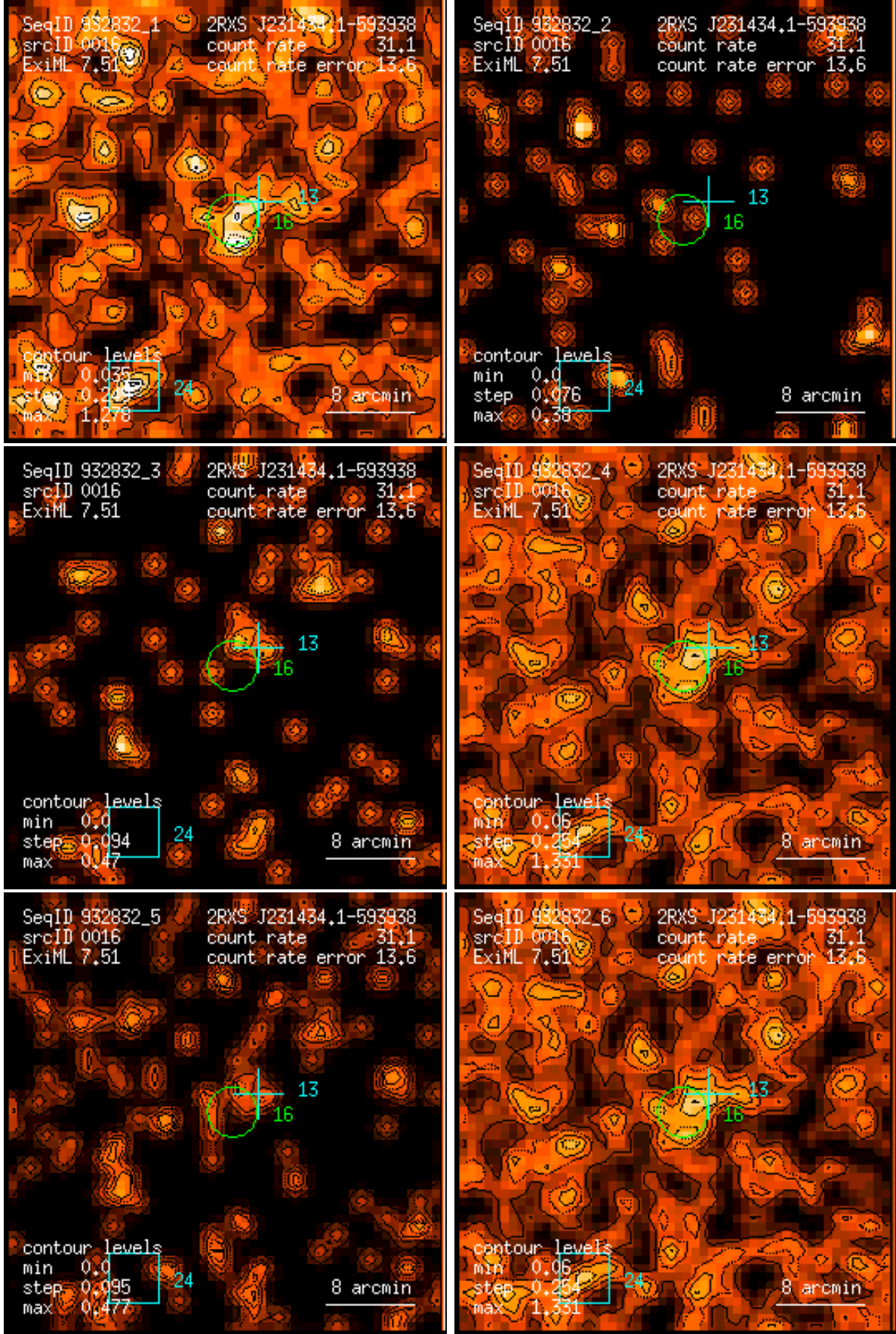
Figure 16: RASS 932832: detection 0016: band rate images, Gaussian filter: (1) PSPC channels 11 – 41, (2) 52 – 90, (3) 91 – 201, (4) 11 – 235, (5) 52 – 201, (6) 11 – 201. Broad band rates in counts/ks. Band rate contour levels in counts/ks/arcmin 2 .
