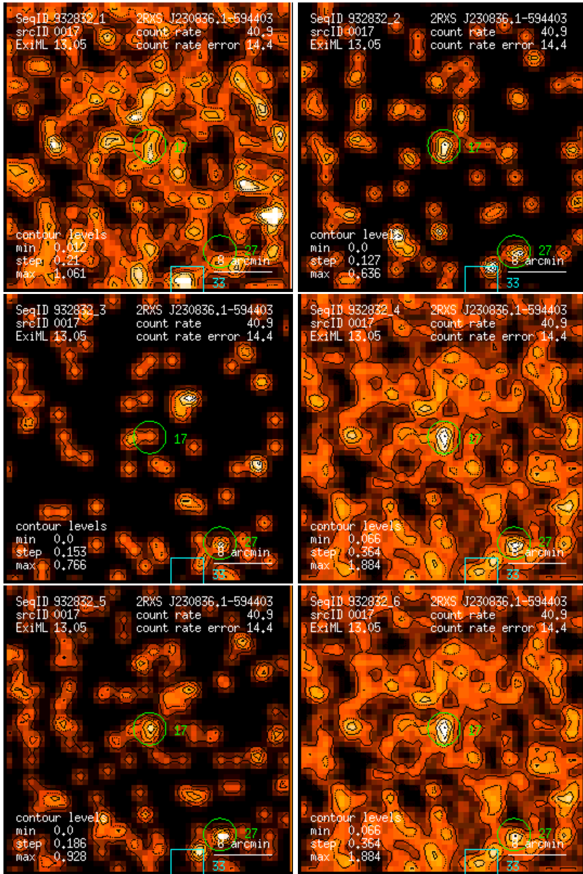
Figure 17: RASS 932832: detection 0017: band rate images, Gaussian filter: (1) PSPC channels 11 – 41, (2) 52 – 90, (3) 91 – 201, (4) 11 – 235, (5) 52 – 201, (6) 11 – 201. Broad band rates in counts/ks. Band rate contour levels in counts/ks/arcmin 2 .
