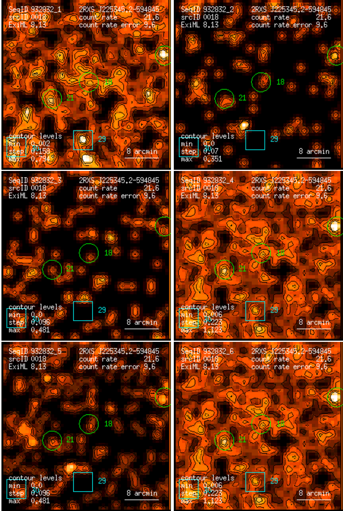
Figure 18: RASS 932832: detection 0018: band rate images, Gaussian filter: (1) PSPC channels 11 – 41, (2) 52 – 90, (3) 91 – 201, (4) 11 – 235, (5) 52 – 201, (6) 11 – 201. Broad band rates in counts/ks. Band rate contour levels in counts/ks/arcmin 2 .
