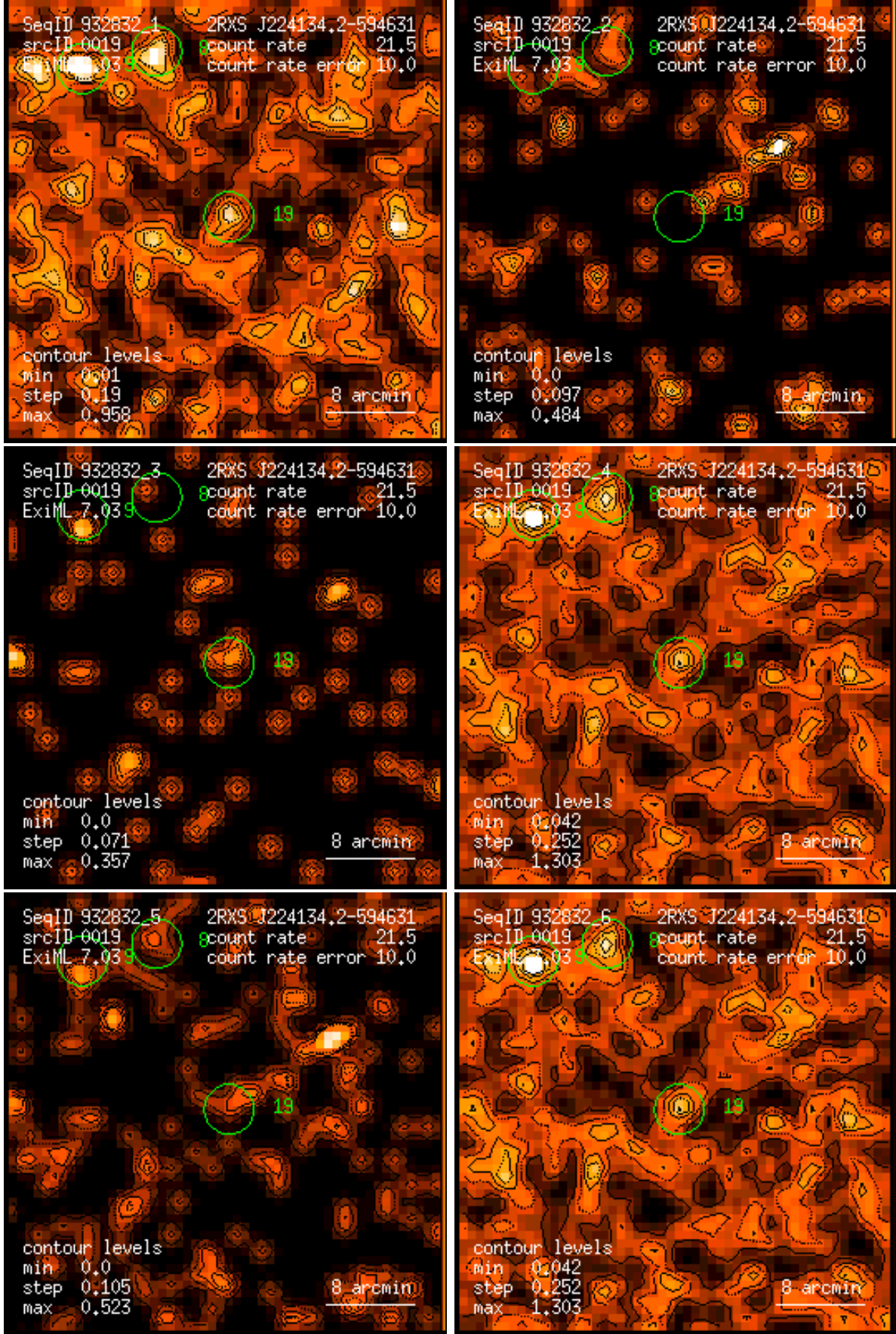
Figure 19: RASS 932832: detection 0019: band rate images, Gaussian filter: (1) PSPC channels 11 – 41, (2) 52 – 90, (3) 91 – 201, (4) 11 – 235, (5) 52 – 201, (6) 11 – 201. Broad band rates in counts/ks. Band rate contour levels in counts/ks/arcmin 2 .
