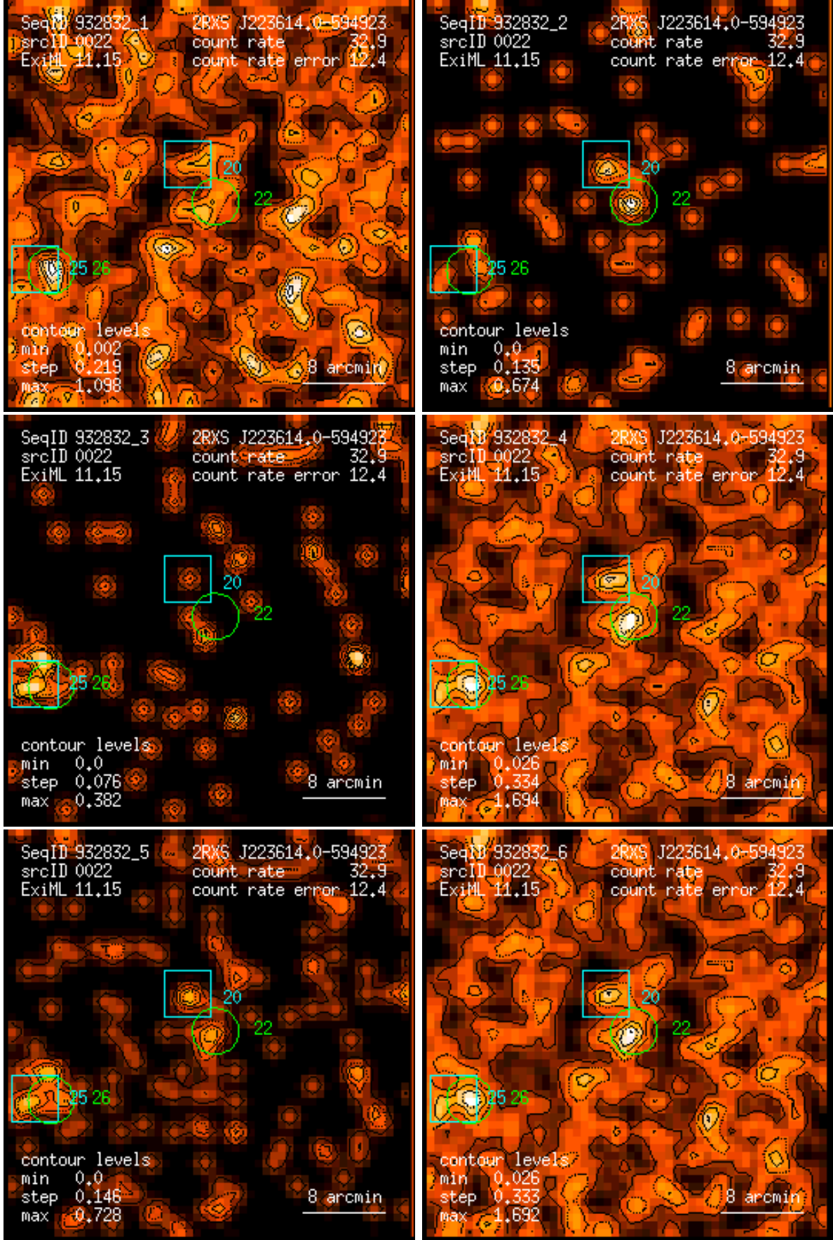
Figure 22: RASS 932832: detection 0022: band rate images, Gaussian filter: (1) PSPC channels 11 – 41, (2) 52 – 90, (3) 91 – 201, (4) 11 – 235, (5) 52 – 201, (6) 11 – 201. Broad band rates in counts/ks. Band rate contour levels in counts/ks/arcmin 2 .
