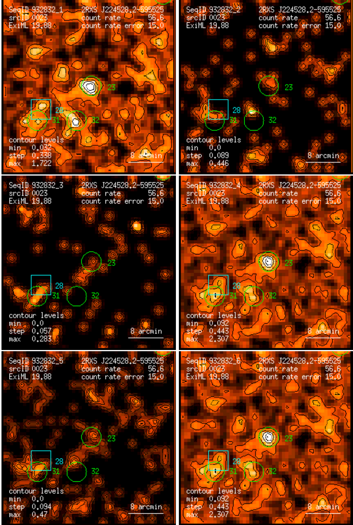
Figure 23: RASS 932832: detection 0023: band rate images, Gaussian filter: (1) PSPC channels 11 – 41, (2) 52 – 90, (3) 91 – 201, (4) 11 – 235, (5) 52 – 201, (6) 11 – 201. Broad band rates in counts/ks. Band rate contour levels in counts/ks/arcmin 2 .
