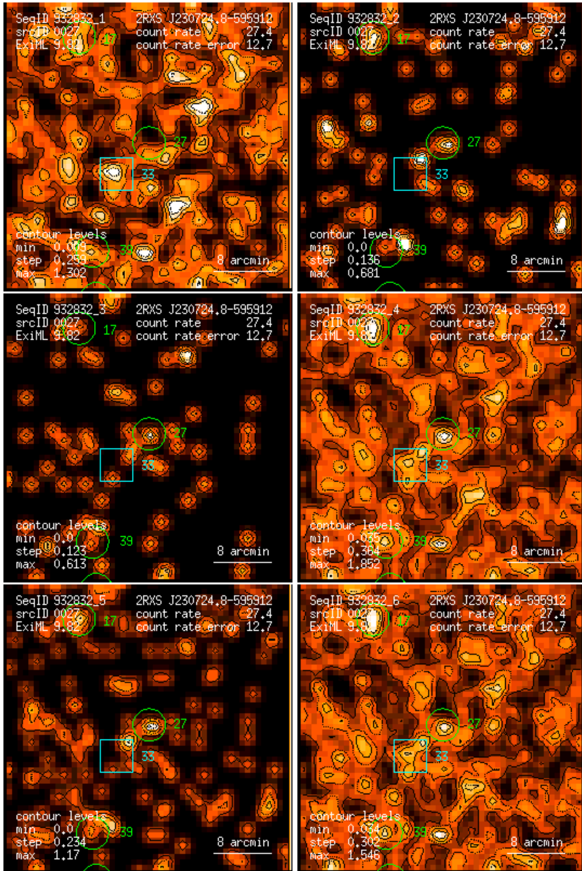
Figure 27: RASS 932832: detection 0027: band rate images, Gaussian filter: (1) PSPC channels 11 – 41, (2) 52 – 90, (3) 91 – 201, (4) 11 – 235, (5) 52 – 201, (6) 11 – 201. Broad band rates in counts/ks. Band rate contour levels in counts/ks/arcmin 2 .
