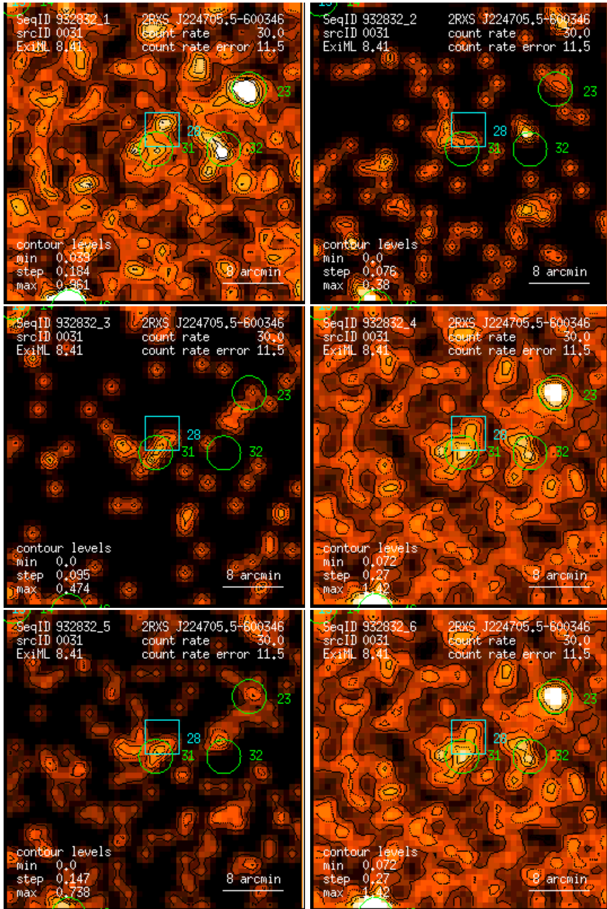
Figure 31: RASS 932832: detection 0031: band rate images, Gaussian filter: (1) PSPC channels 11 – 41, (2) 52 – 90, (3) 91 – 201, (4) 11 – 235, (5) 52 – 201, (6) 11 – 201. Broad band rates in counts/ks. Band rate contour levels in counts/ks/arcmin 2 .
