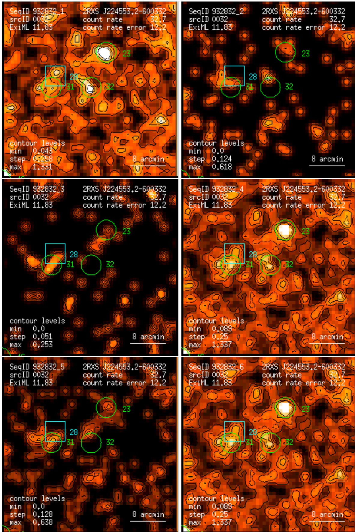
Figure 32: RASS 932832: detection 0032: band rate images, Gaussian filter: (1) PSPC channels 11 – 41, (2) 52 – 90, (3) 91 – 201, (4) 11 – 235, (5) 52 – 201, (6) 11 – 201. Broad band rates in counts/ks. Band rate contour levels in counts/ks/arcmin 2 .
