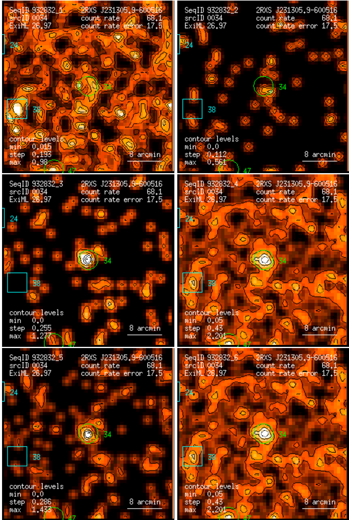
Figure 34: RASS 932832: detection 0034: band rate images, Gaussian filter: (1) PSPC channels 11 – 41, (2) 52 – 90, (3) 91 – 201, (4) 11 – 235, (5) 52 – 201, (6) 11 – 201. Broad band rates in counts/ks. Band rate contour levels in counts/ks/arcmin 2 .
