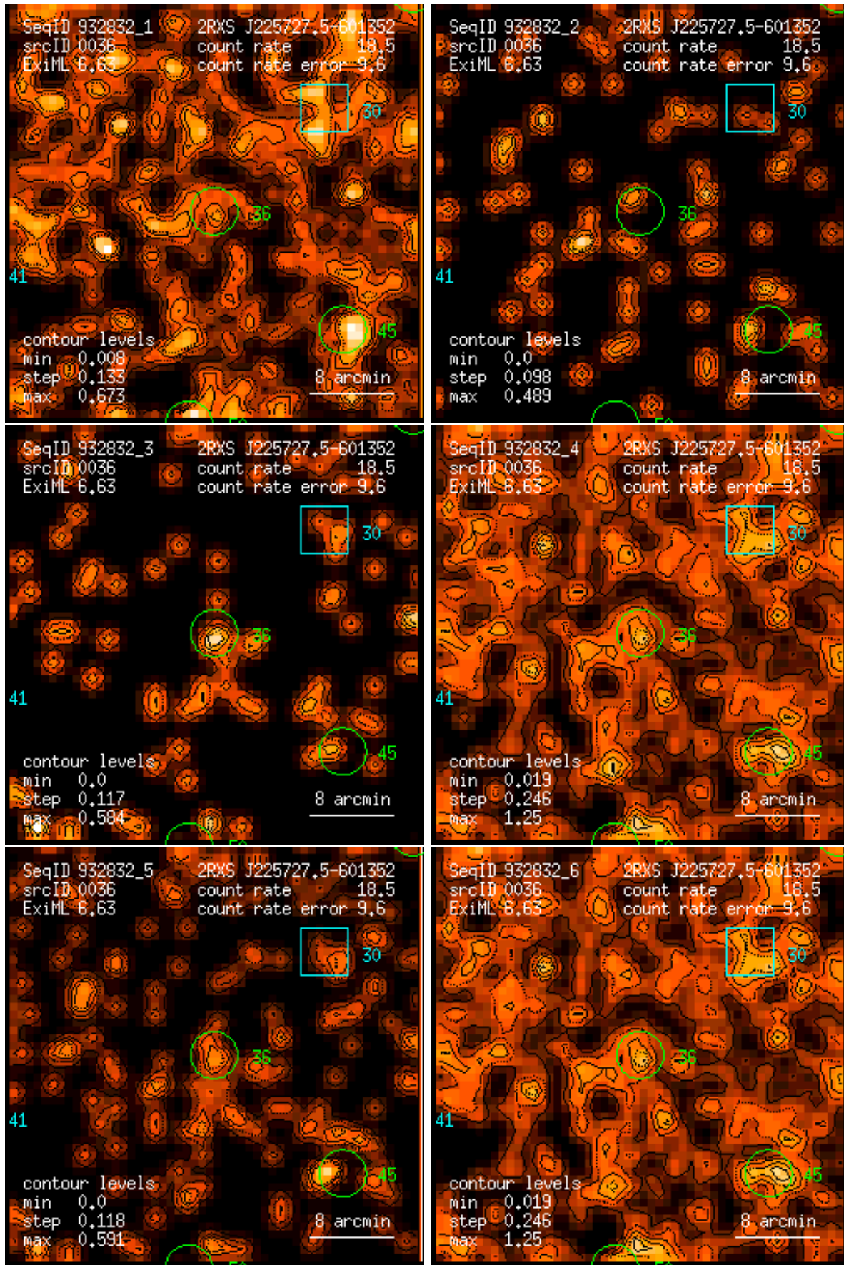
Figure 36: RASS 932832: detection 0036: band rate images, Gaussian filter: (1) PSPC channels 11 – 41, (2) 52 – 90, (3) 91 – 201, (4) 11 – 235, (5) 52 – 201, (6) 11 – 201. Broad band rates in counts/ks. Band rate contour levels in counts/ks/arcmin 2 .
