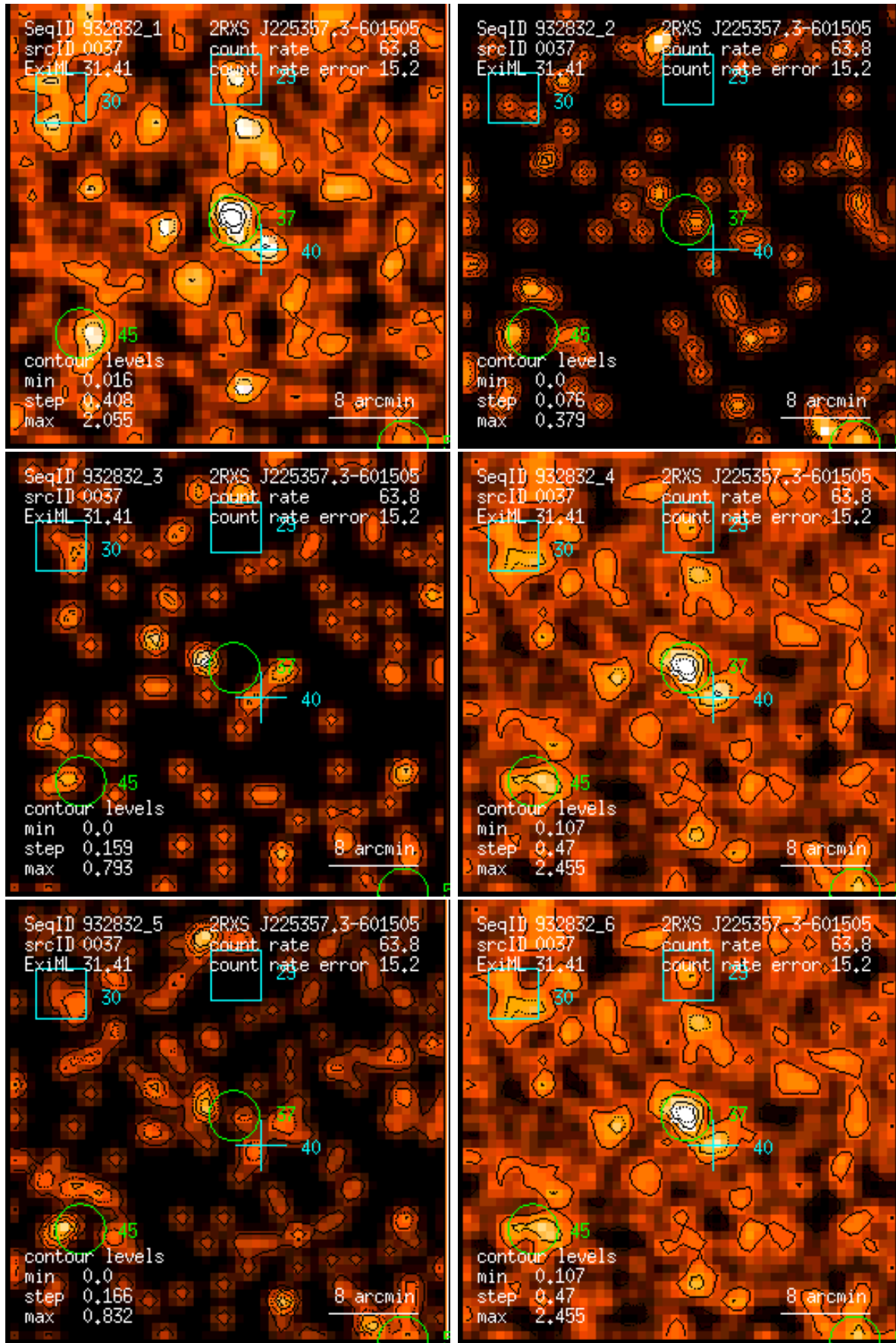
Figure 37: RASS 932832: detection 0037: band rate images, Gaussian filter: (1) PSPC channels 11 – 41, (2) 52 – 90, (3) 91 – 201, (4) 11 – 235, (5) 52 – 201, (6) 11 – 201. Broad band rates in counts/ks. Band rate contour levels in counts/ks/arcmin 2 .
