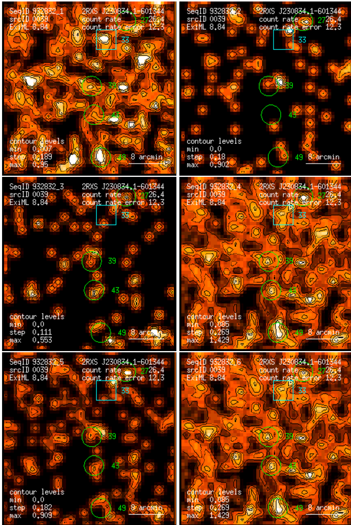
Figure 39: RASS 932832: detection 0039: band rate images, Gaussian filter: (1) PSPC channels 11 – 41, (2) 52 – 90, (3) 91 – 201, (4) 11 – 235, (5) 52 – 201, (6) 11 – 201. Broad band rates in counts/ks. Band rate contour levels in counts/ks/arcmin 2 .
