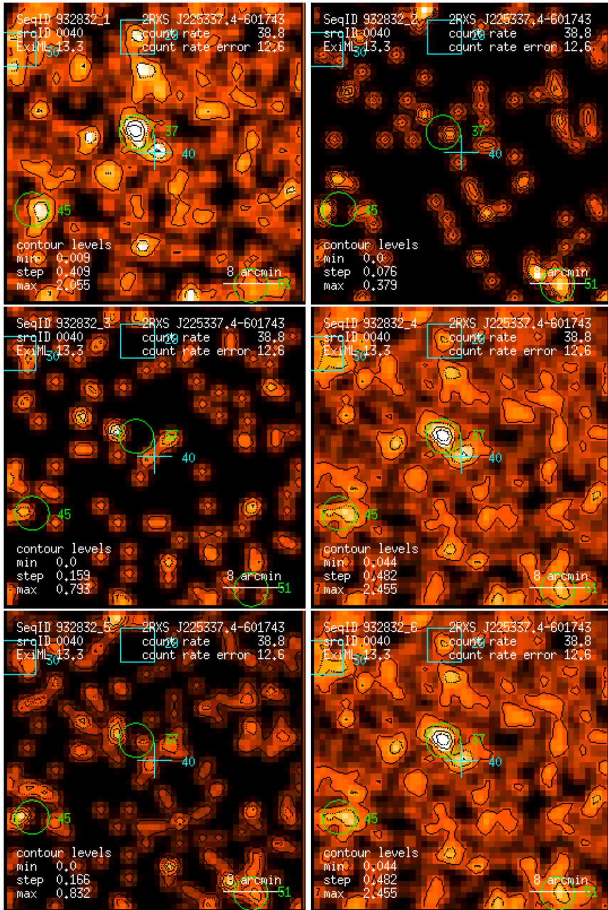
Figure 40: RASS 932832: detection 0040: band rate images, Gaussian filter: (1) PSPC channels 11 – 41, (2) 52 – 90, (3) 91 – 201, (4) 11 – 235, (5) 52 – 201, (6) 11 – 201. Broad band rates in counts/ks. Band rate contour levels in counts/ks/arcmin 2 .
