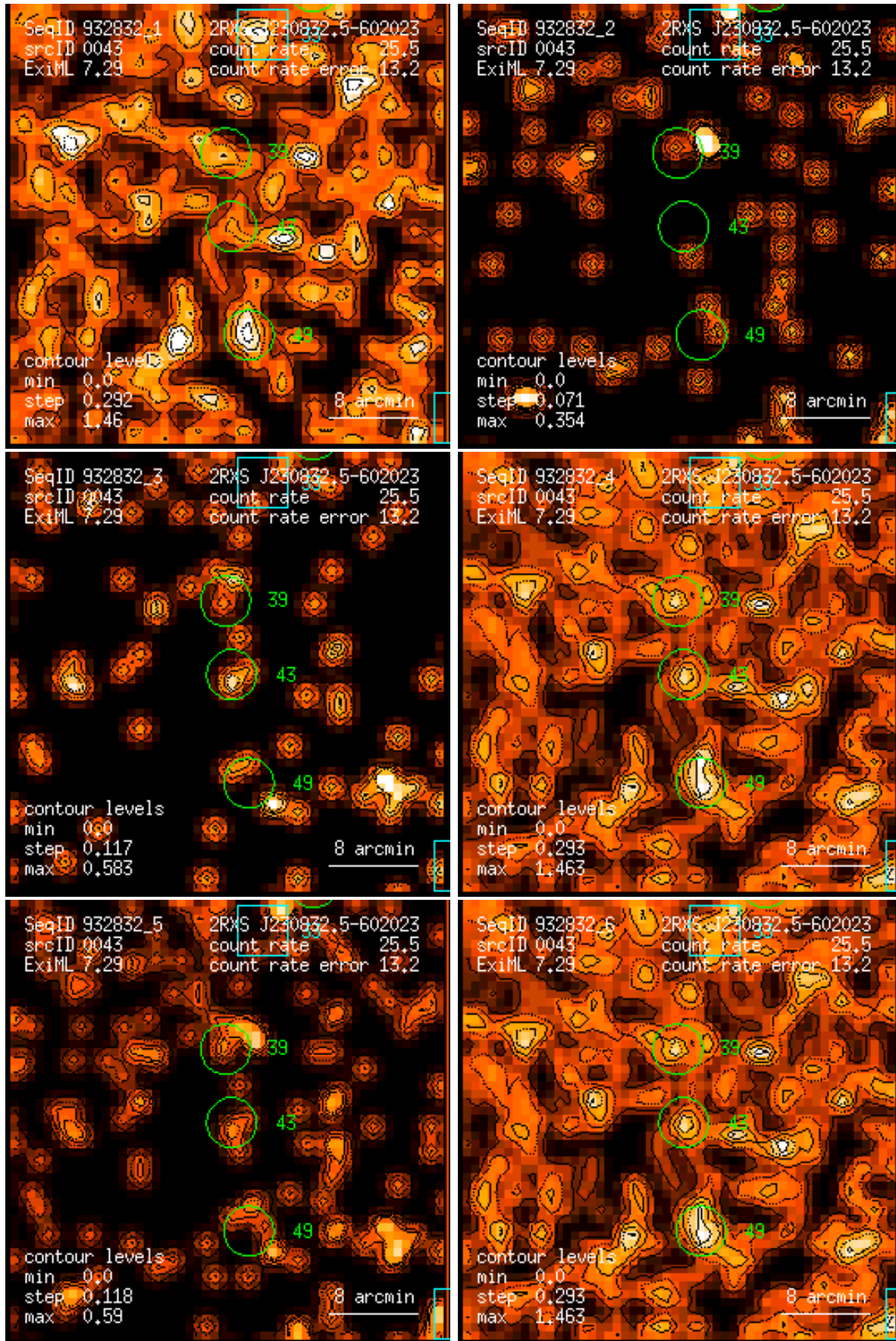
Figure 43: RASS 932832: detection 0043: band rate images, Gaussian filter: (1) PSPC channels 11 – 41, (2) 52 – 90, (3) 91 – 201, (4) 11 – 235, (5) 52 – 201, (6) 11 – 201. Broad band rates in counts/ks. Band rate contour levels in counts/ks/arcmin 2 .
