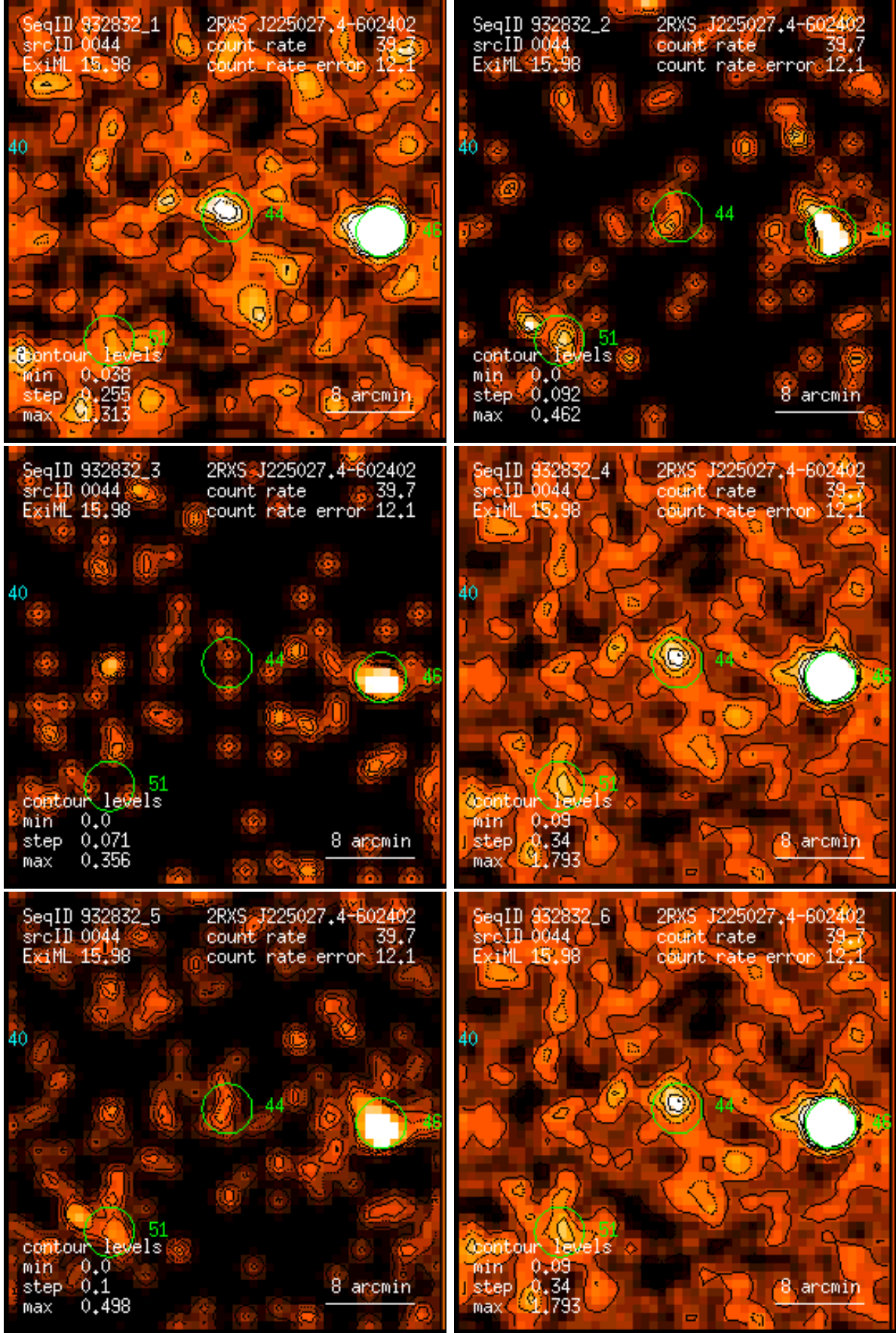
Figure 44: RASS 932832: detection 0044: band rate images, Gaussian filter: (1) PSPC channels 11 – 41, (2) 52 – 90, (3) 91 – 201, (4) 11 – 235, (5) 52 – 201, (6) 11 – 201. Broad band rates in counts/ks. Band rate contour levels in counts/ks/arcmin 2 .
