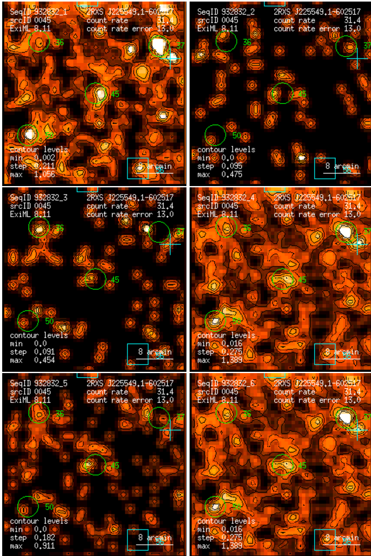
Figure 45: RASS 932832: detection 0045: band rate images, Gaussian filter: (1) PSPC channels 11 – 41, (2) 52 – 90, (3) 91 – 201, (4) 11 – 235, (5) 52 – 201, (6) 11 – 201. Broad band rates in counts/ks. Band rate contour levels in counts/ks/arcmin 2 .
