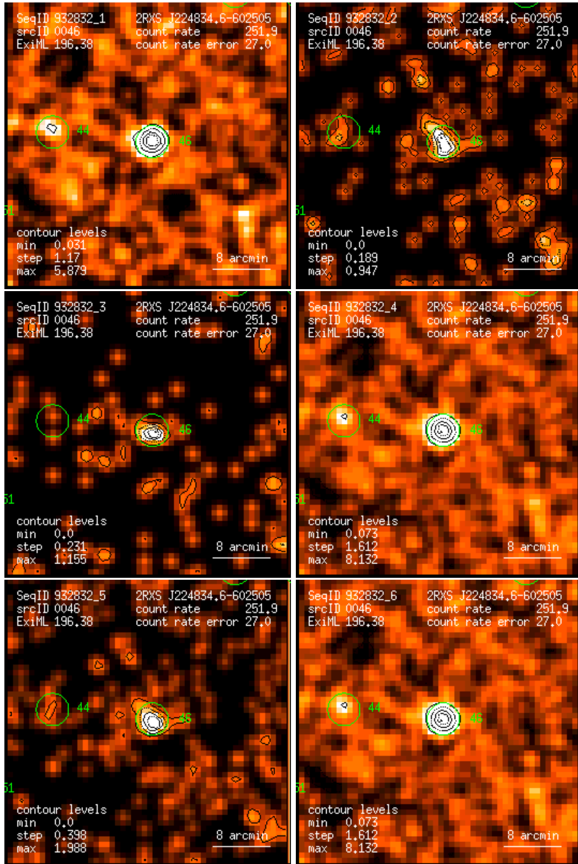
Figure 46: RASS 932832: detection 0046: band rate images, Gaussian filter: (1) PSPC channels 11 – 41, (2) 52 – 90, (3) 91 – 201, (4) 11 – 235, (5) 52 – 201, (6) 11 – 201. Broad band rates in counts/ks. Band rate contour levels in counts/ks/arcmin 2 .
