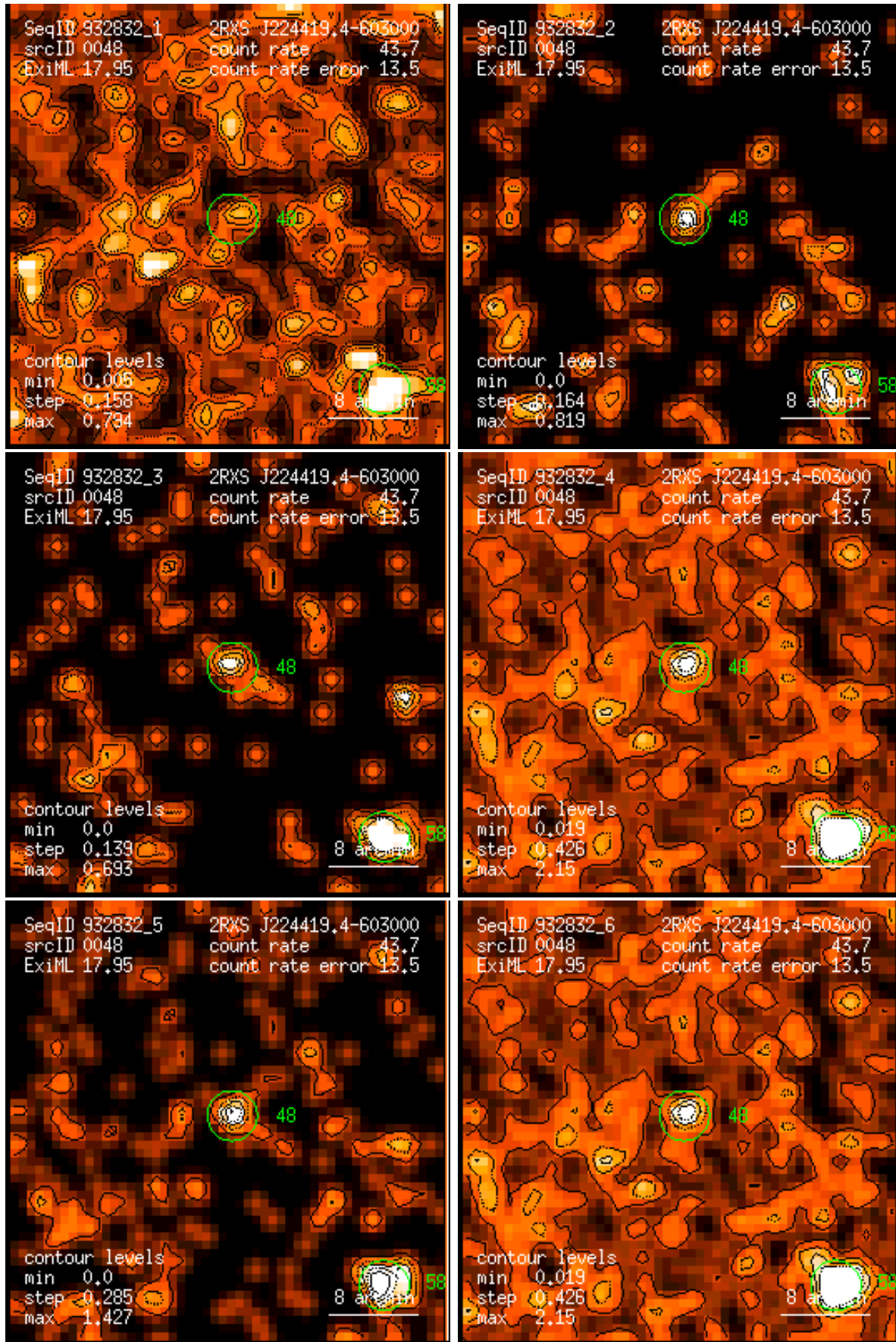
Figure 48: RASS 932832: detection 0048: band rate images, Gaussian filter: (1) PSPC channels 11 – 41, (2) 52 – 90, (3) 91 – 201, (4) 11 – 235, (5) 52 – 201, (6) 11 – 201. Broad band rates in counts/ks. Band rate contour levels in counts/ks/arcmin 2 .
