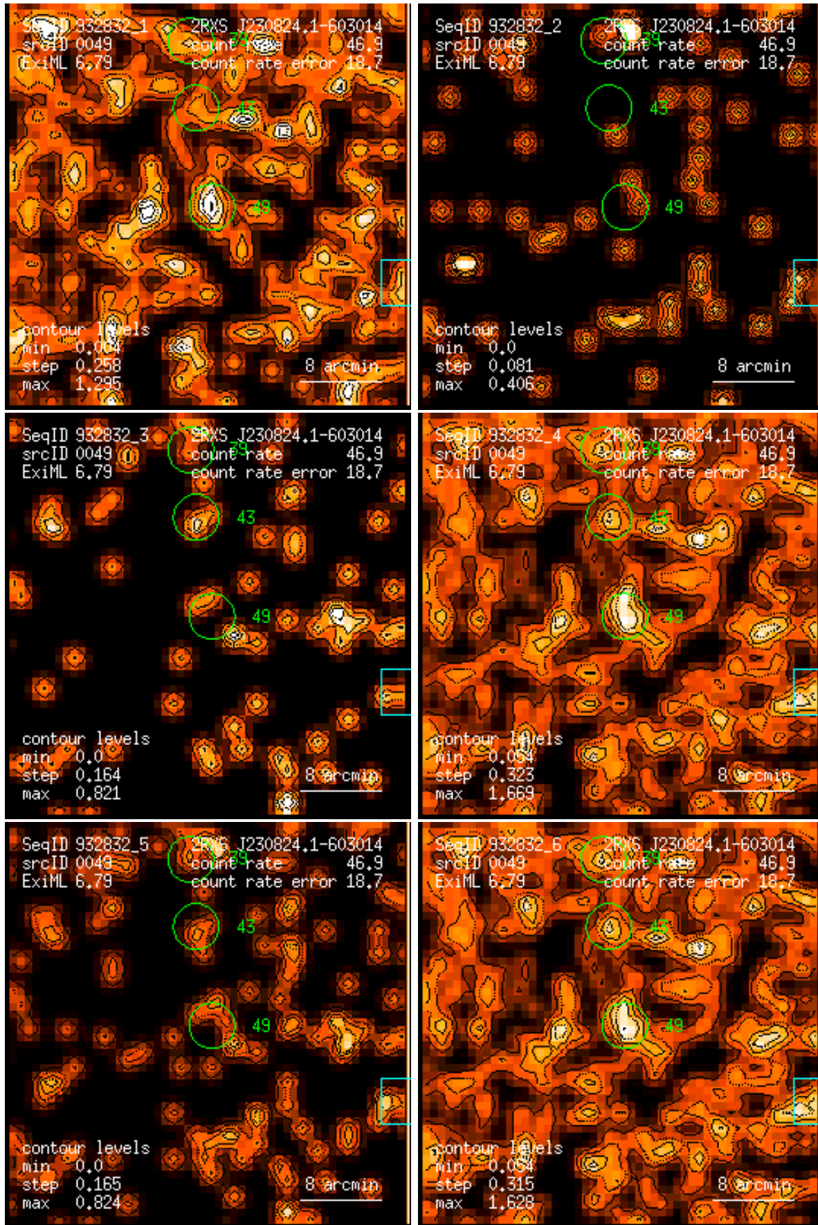
Figure 49: RASS 932832: detection 0049: band rate images, Gaussian filter: (1) PSPC channels 11 – 41, (2) 52 – 90, (3) 91 – 201, (4) 11 – 235, (5) 52 – 201, (6) 11 – 201. Broad band rates in counts/ks. Band rate contour levels in counts/ks/arcmin 2 .
