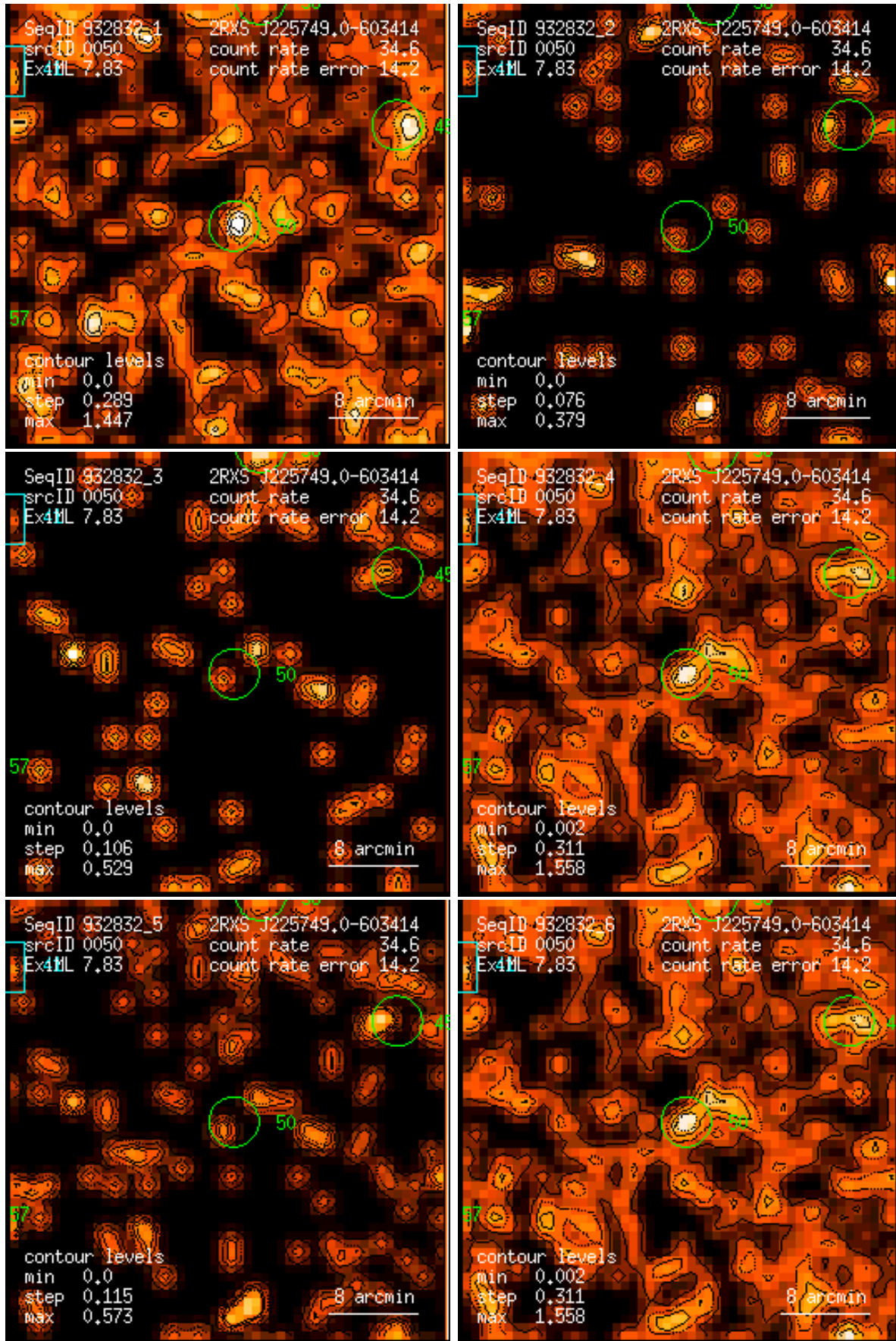
Figure 50: RASS 932832: detection 0050: band rate images, Gaussian filter: (1) PSPC channels 11 – 41, (2) 52 – 90, (3) 91 – 201, (4) 11 – 235, (5) 52 – 201, (6) 11 – 201. Broad band rates in counts/ks. Band rate contour levels in counts/ks/arcmin 2 .
