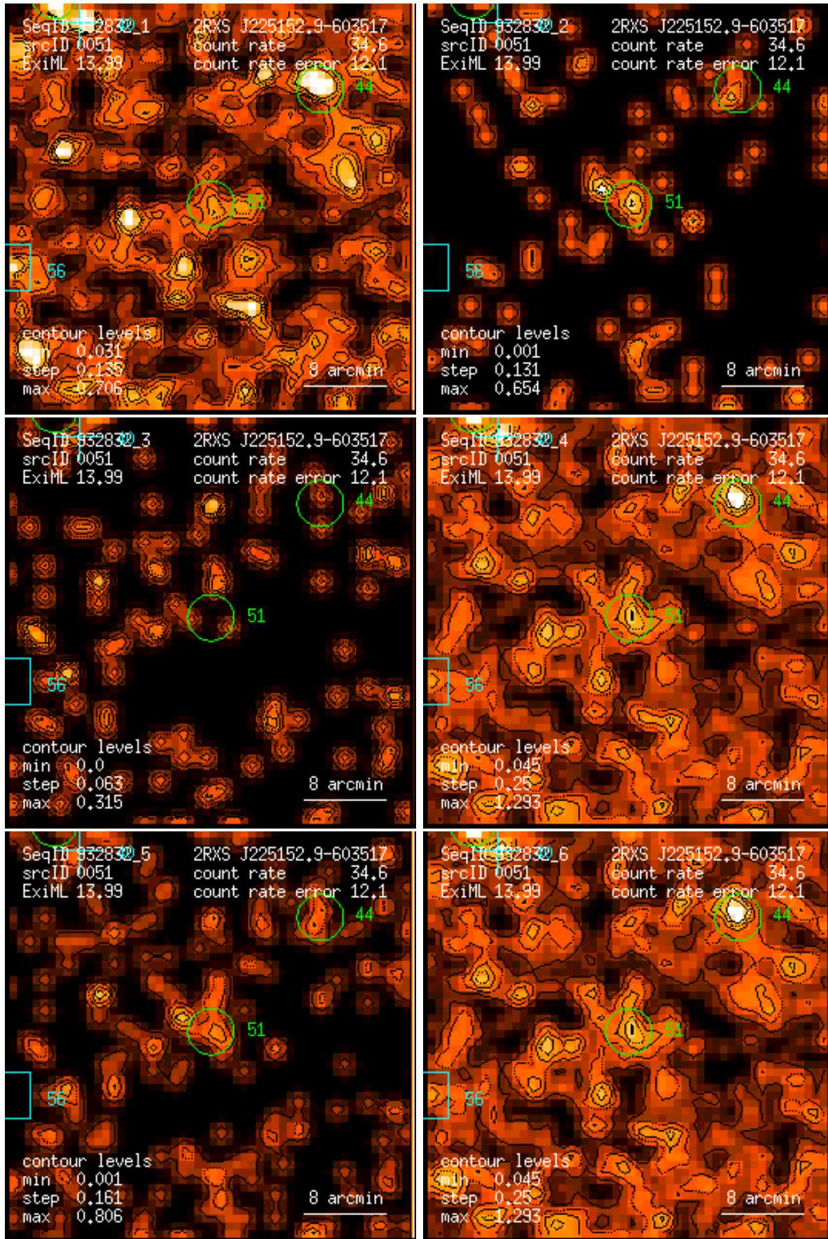
Figure 51: RASS 932832: detection 0051: band rate images, Gaussian filter: (1) PSPC channels 11 – 41, (2) 52 – 90, (3) 91 – 201, (4) 11 – 235, (5) 52 – 201, (6) 11 – 201. Broad band rates in counts/ks. Band rate contour levels in counts/ks/arcmin 2 .
