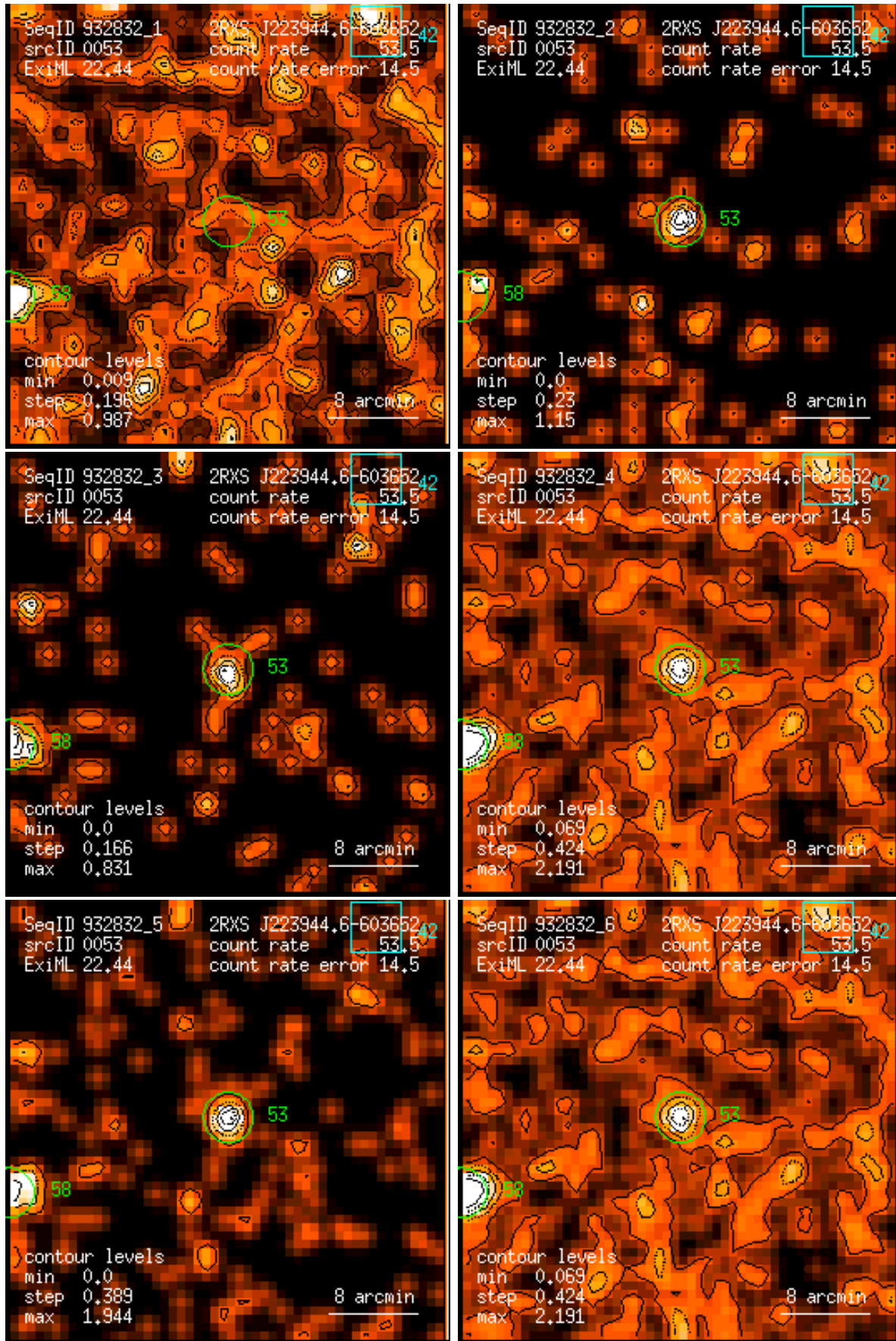
Figure 53: RASS 932832: detection 0053: band rate images, Gaussian filter: (1) PSPC channels 11 – 41, (2) 52 – 90, (3) 91 – 201, (4) 11 – 235, (5) 52 – 201, (6) 11 – 201. Broad band rates in counts/ks. Band rate contour levels in counts/ks/arcmin 2 .
