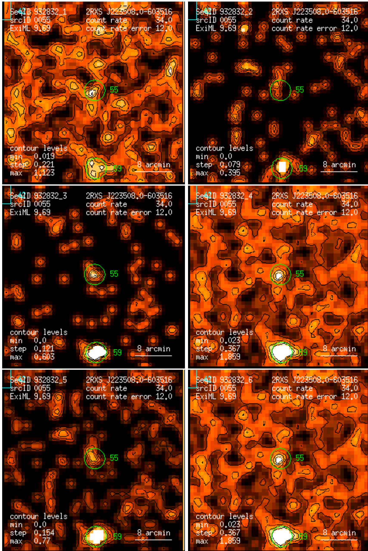
Figure 55: RASS 932832: detection 0055: band rate images, Gaussian filter: (1) PSPC channels 11 – 41, (2) 52 – 90, (3) 91 – 201, (4) 11 – 235, (5) 52 – 201, (6) 11 – 201. Broad band rates in counts/ks. Band rate contour levels in counts/ks/arcmin 2 .
