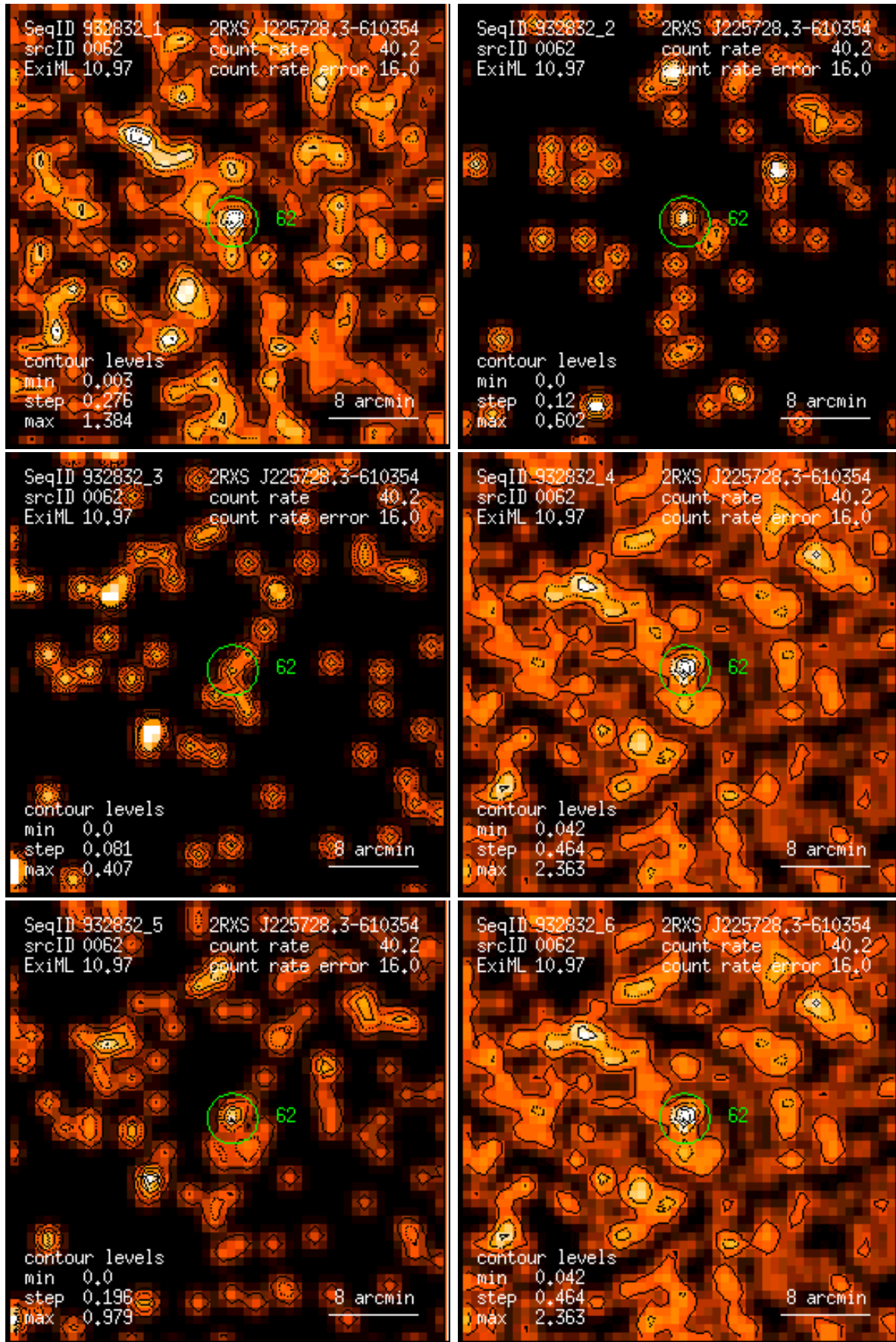
Figure 62: RASS 932832: detection 0062: band rate images, Gaussian filter: (1) PSPC channels 11 – 41, (2) 52 – 90, (3) 91 – 201, (4) 11 – 235, (5) 52 – 201, (6) 11 – 201. Broad band rates in counts/ks. Band rate contour levels in counts/ks/arcmin 2 .
