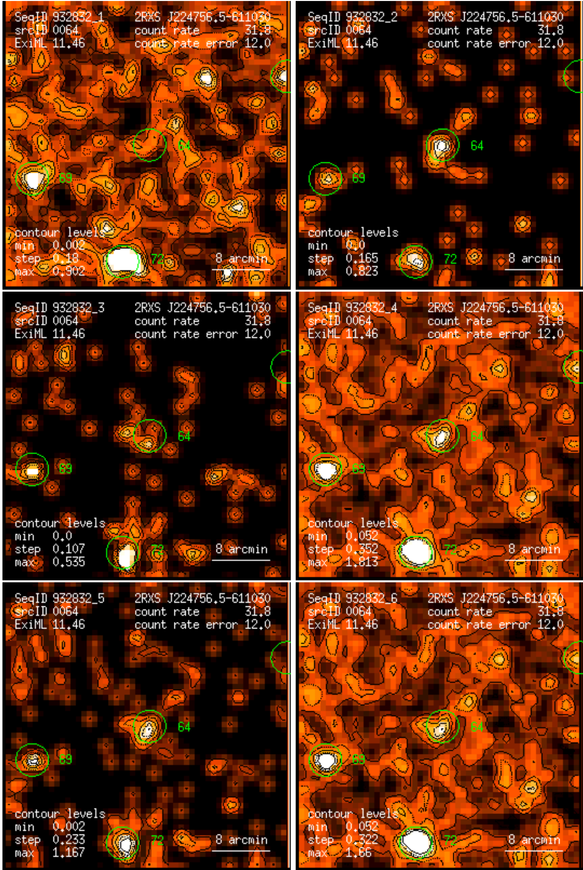
Figure 64: RASS 932832: detection 0064: band rate images, Gaussian filter: (1) PSPC channels 11 – 41, (2) 52 – 90, (3) 91 – 201, (4) 11 – 235, (5) 52 – 201, (6) 11 – 201. Broad band rates in counts/ks. Band rate contour levels in counts/ks/arcmin 2 .
