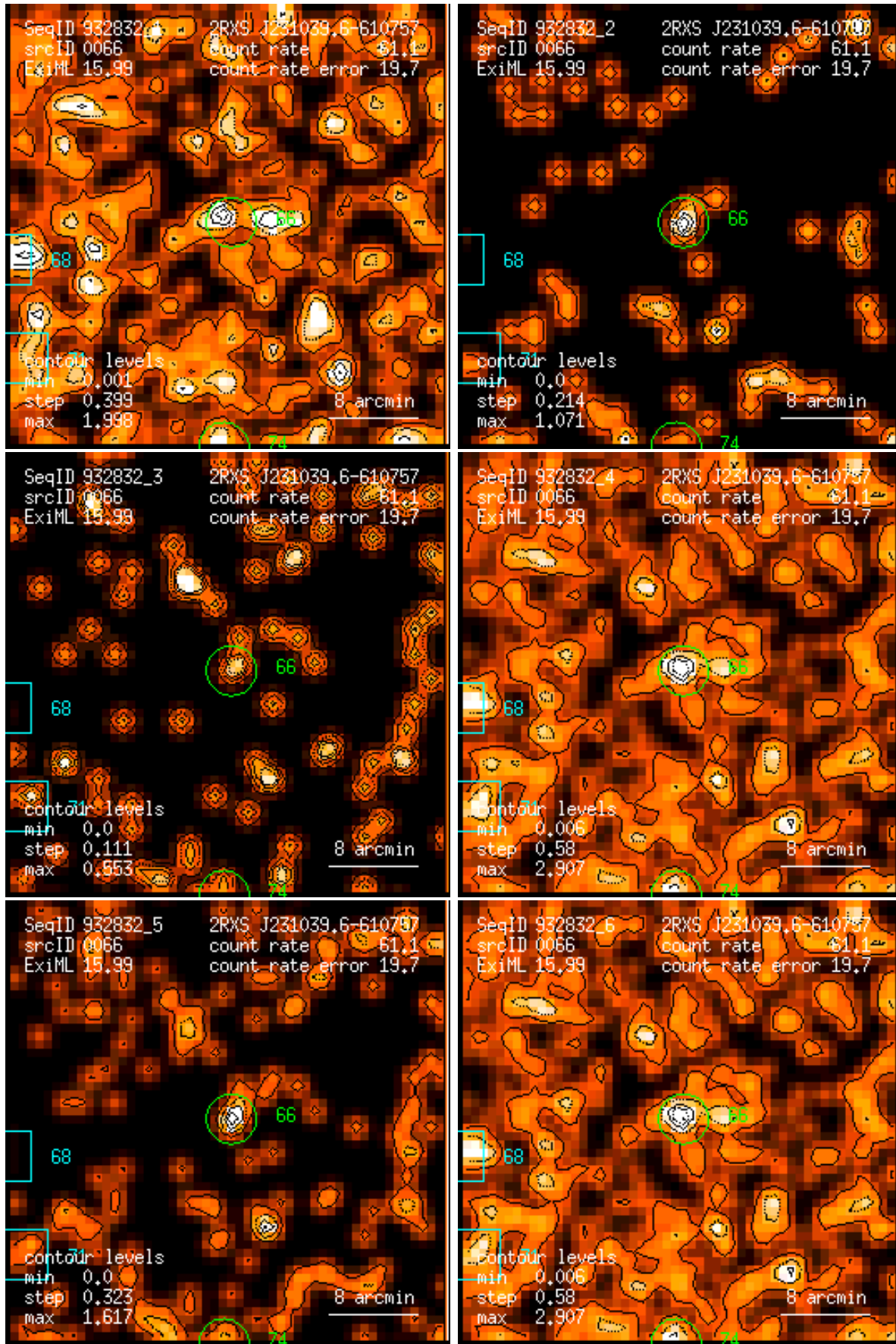
Figure 66: RASS 932832: detection 0066: band rate images, Gaussian filter: (1) PSPC channels 11 – 41, (2) 52 – 90, (3) 91 – 201, (4) 11 – 235, (5) 52 – 201, (6) 11 – 201. Broad band rates in counts/ks. Band rate contour levels in counts/ks/arcmin 2 .
