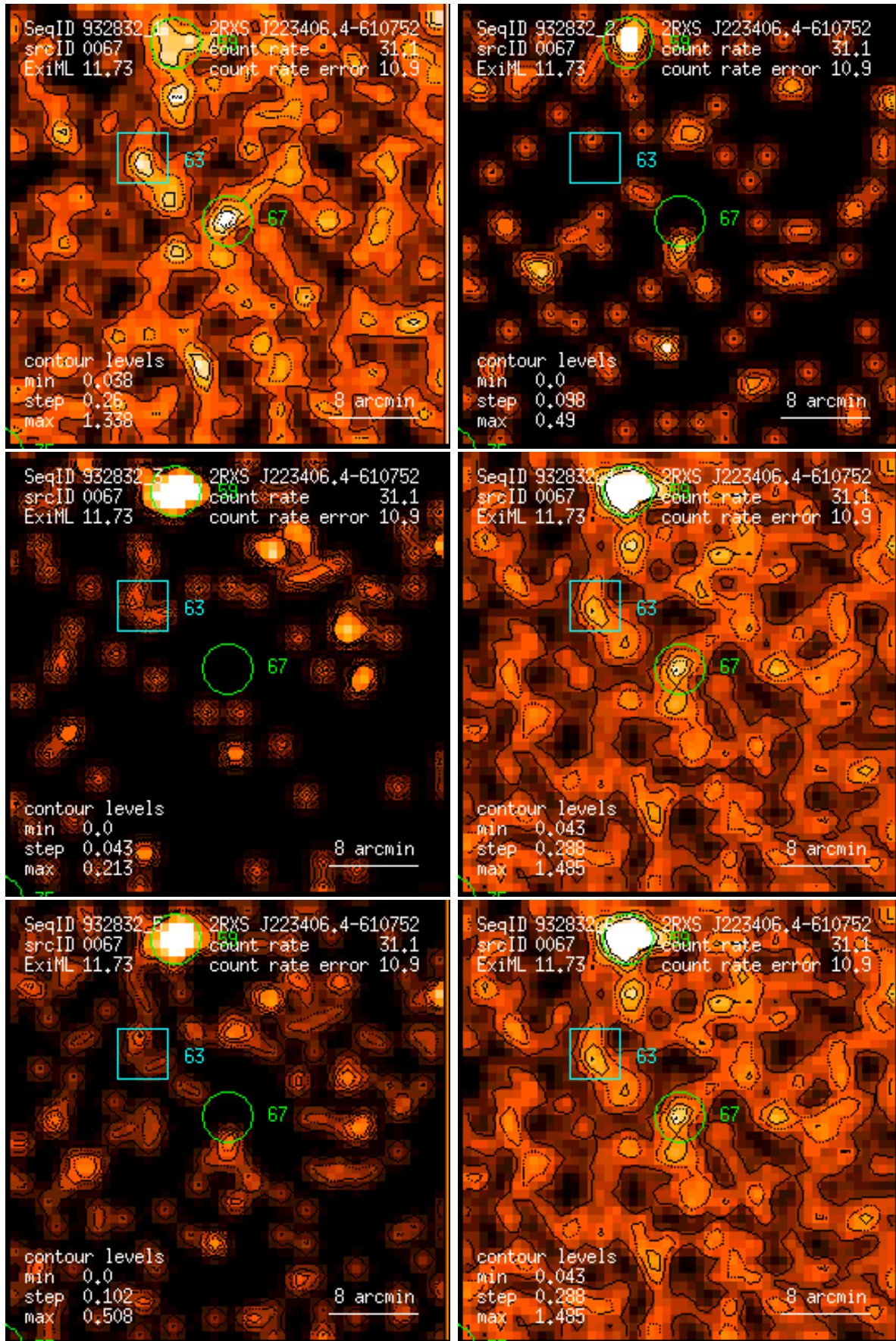
Figure 67: RASS 932832: detection 0067: band rate images, Gaussian filter: (1) PSPC channels 11 – 41, (2) 52 – 90, (3) 91 – 201, (4) 11 – 235, (5) 52 – 201, (6) 11 – 201. Broad band rates in counts/ks. Band rate contour levels in counts/ks/arcmin 2 .
