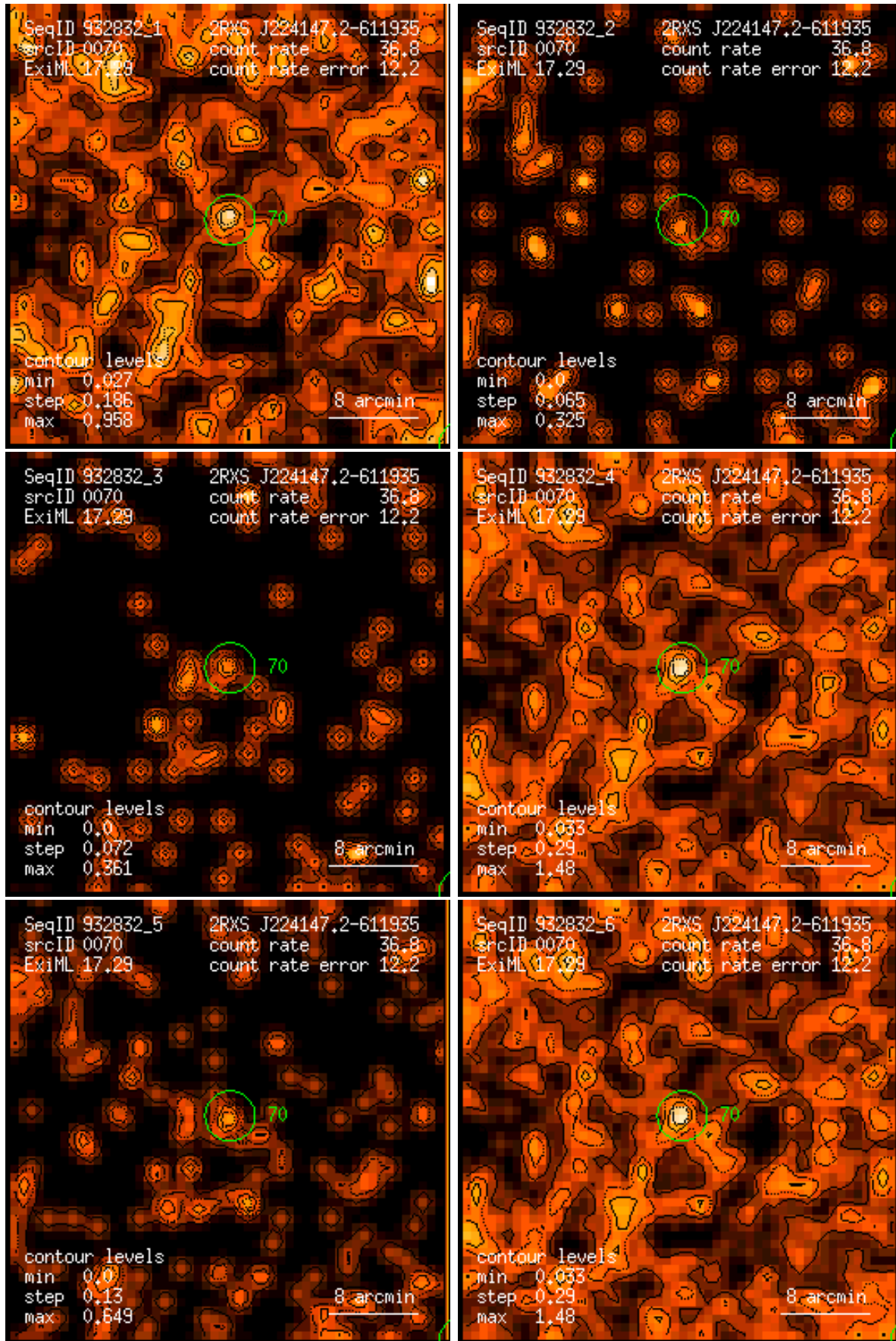
Figure 70: RASS 932832: detection 0070: band rate images, Gaussian filter: (1) PSPC channels 11 – 41, (2) 52 – 90, (3) 91 – 201, (4) 11 – 235, (5) 52 – 201, (6) 11 – 201. Broad band rates in counts/ks. Band rate contour levels in counts/ks/arcmin 2 .
