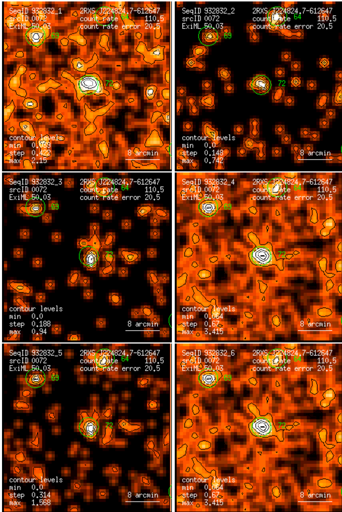
Figure 72: RASS 932832: detection 0072: band rate images, Gaussian filter: (1) PSPC channels 11 – 41, (2) 52 – 90, (3) 91 – 201, (4) 11 – 235, (5) 52 – 201, (6) 11 – 201. Broad band rates in counts/ks. Band rate contour levels in counts/ks/arcmin 2 .
