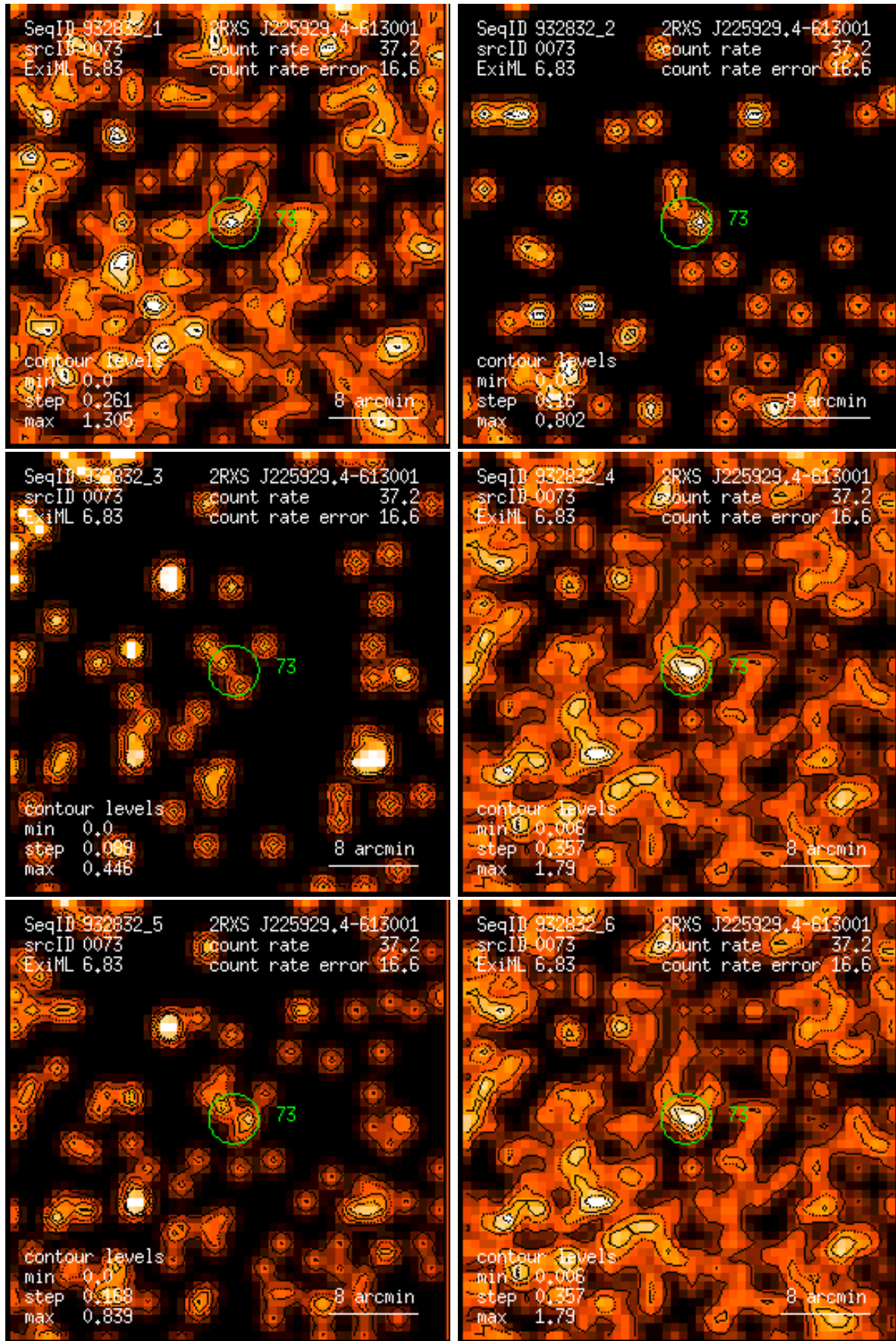
Figure 73: RASS 932832: detection 0073: band rate images, Gaussian filter: (1) PSPC channels 11 – 41, (2) 52 – 90, (3) 91 – 201, (4) 11 – 235, (5) 52 – 201, (6) 11 – 201. Broad band rates in counts/ks. Band rate contour levels in counts/ks/arcmin 2 .
