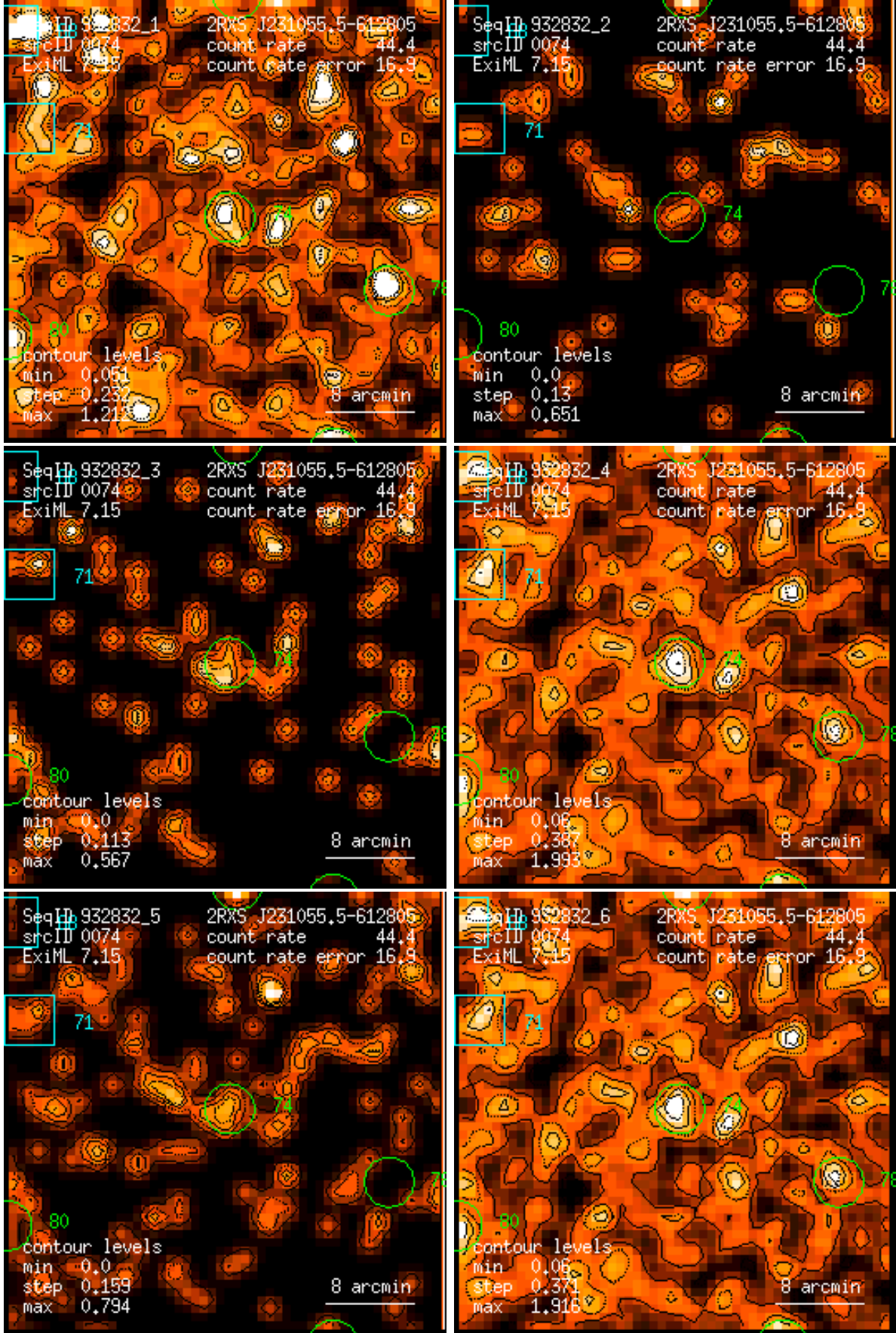
Figure 74: RASS 932832: detection 0074: band rate images, Gaussian filter: (1) PSPC channels 11 – 41, (2) 52 – 90, (3) 91 – 201, (4) 11 – 235, (5) 52 – 201, (6) 11 – 201. Broad band rates in counts/ks. Band rate contour levels in counts/ks/arcmin 2 .
