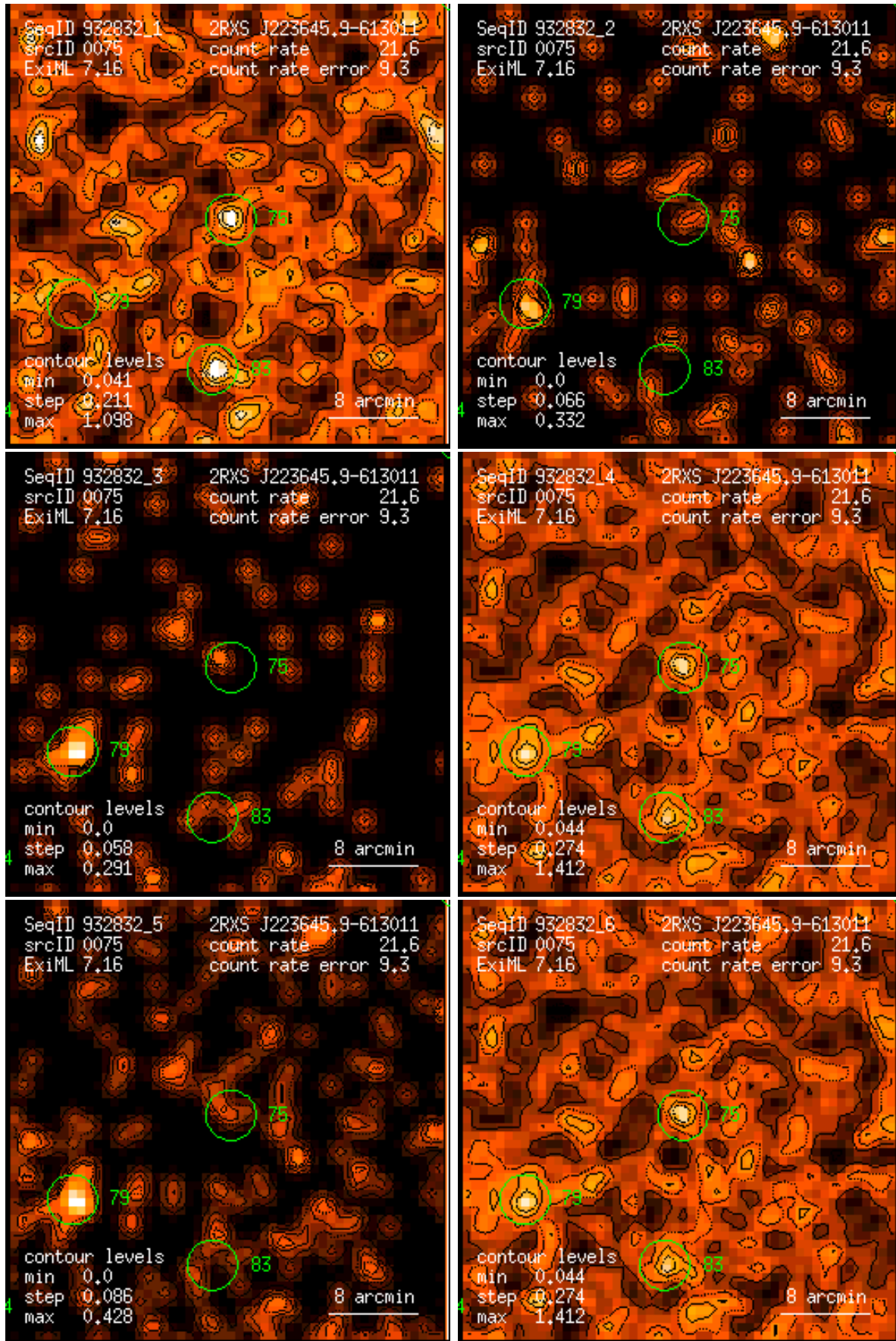
Figure 75: RASS 932832: detection 0075: band rate images, Gaussian filter: (1) PSPC channels 11 – 41, (2) 52 – 90, (3) 91 – 201, (4) 11 – 235, (5) 52 – 201, (6) 11 – 201. Broad band rates in counts/ks. Band rate contour levels in counts/ks/arcmin 2 .
