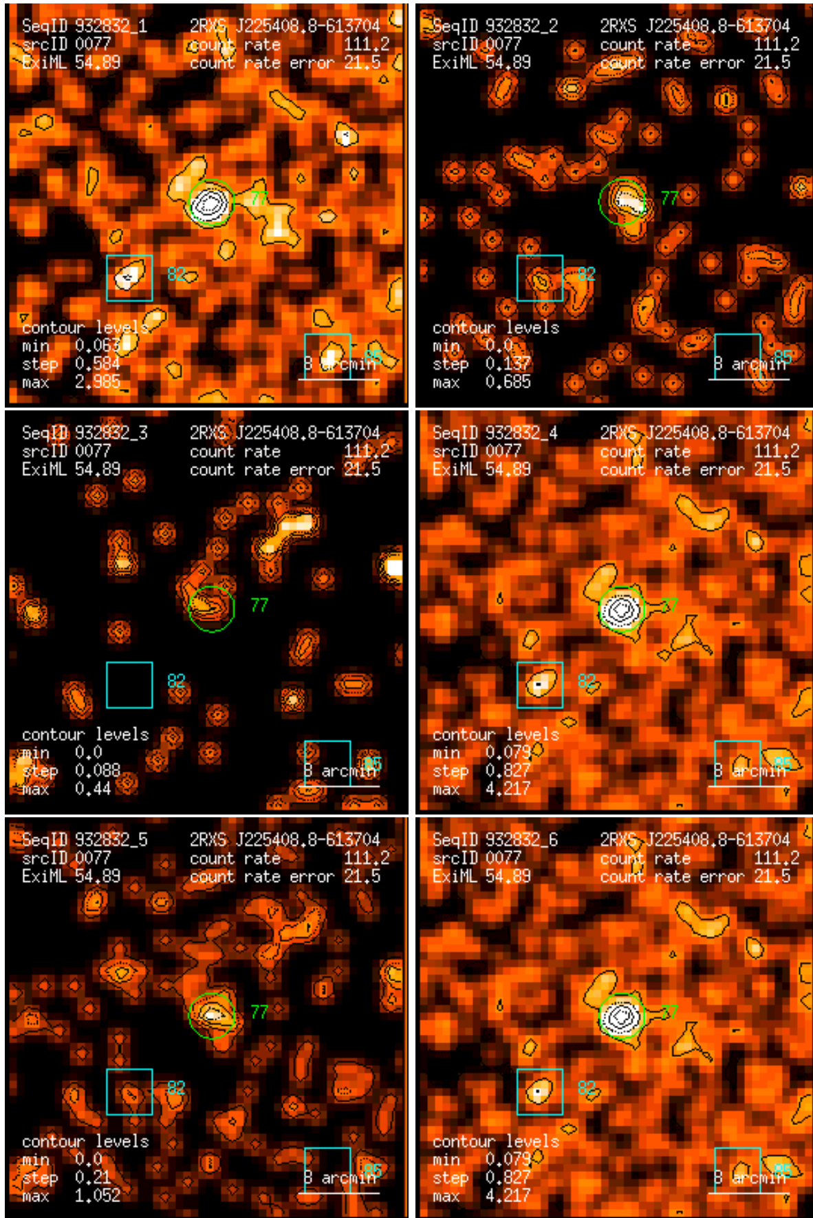
Figure 77: RASS 932832: detection 0077: band rate images, Gaussian filter: (1) PSPC channels 11 – 41, (2) 52 – 90, (3) 91 – 201, (4) 11 – 235, (5) 52 – 201, (6) 11 – 201. Broad band rates in counts/ks. Band rate contour levels in counts/ks/arcmin 2 .
