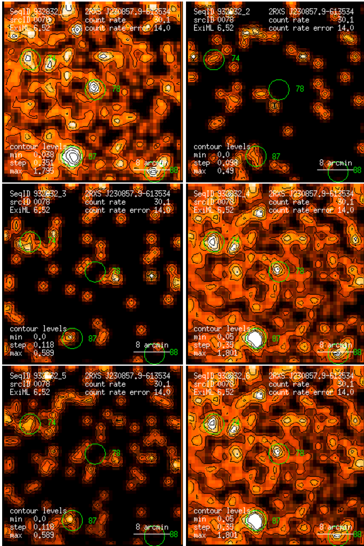
Figure 78: RASS 932832: detection 0078: band rate images, Gaussian filter: (1) PSPC channels 11 – 41, (2) 52 – 90, (3) 91 – 201, (4) 11 – 235, (5) 52 – 201, (6) 11 – 201. Broad band rates in counts/ks. Band rate contour levels in counts/ks/arcmin 2 .
