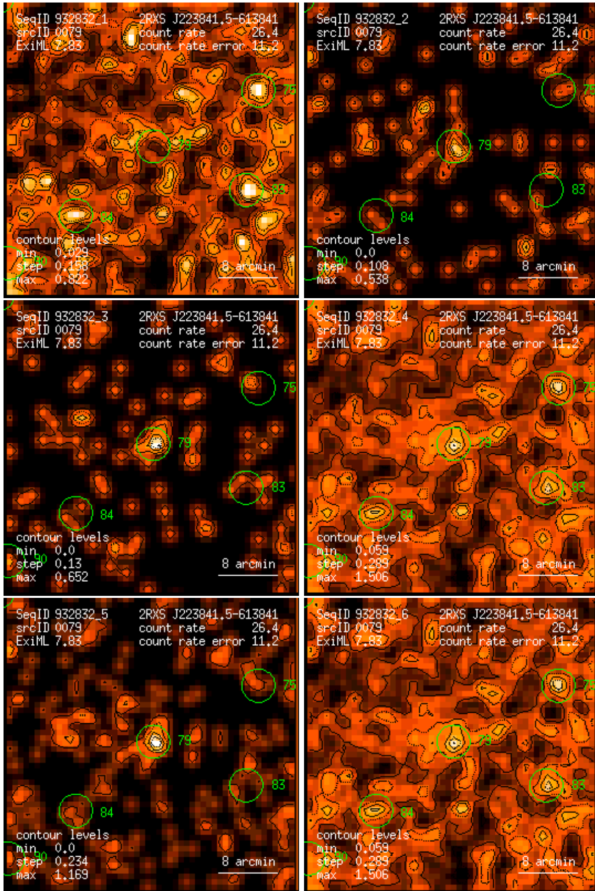
Figure 79: RASS 932832: detection 0079: band rate images, Gaussian filter: (1) PSPC channels 11 – 41, (2) 52 – 90, (3) 91 – 201, (4) 11 – 235, (5) 52 – 201, (6) 11 – 201. Broad band rates in counts/ks. Band rate contour levels in counts/ks/arcmin 2 .
