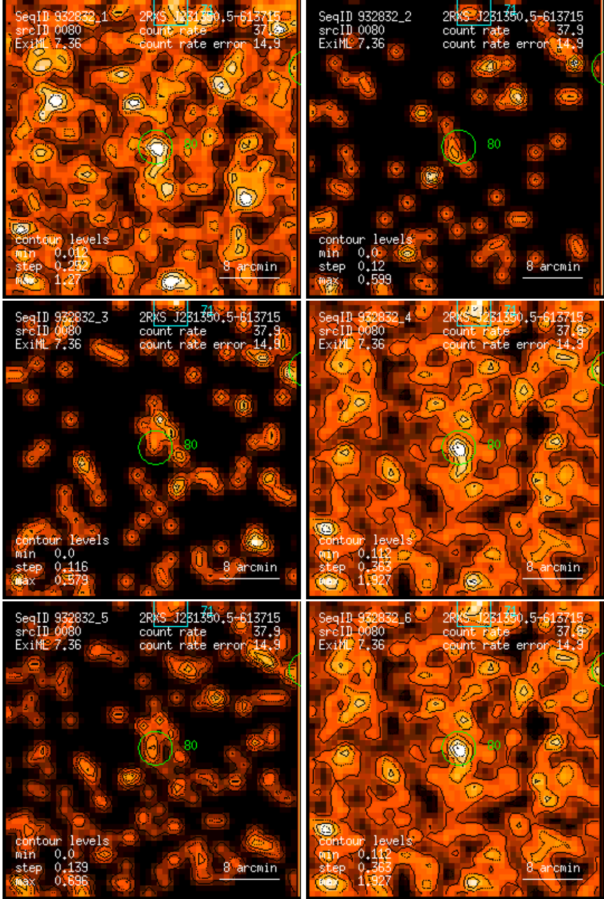
Figure 80: RASS 932832: detection 0080: band rate images, Gaussian filter: (1) PSPC channels 11 – 41, (2) 52 – 90, (3) 91 – 201, (4) 11 – 235, (5) 52 – 201, (6) 11 – 201. Broad band rates in counts/ks. Band rate contour levels in counts/ks/arcmin 2 .
