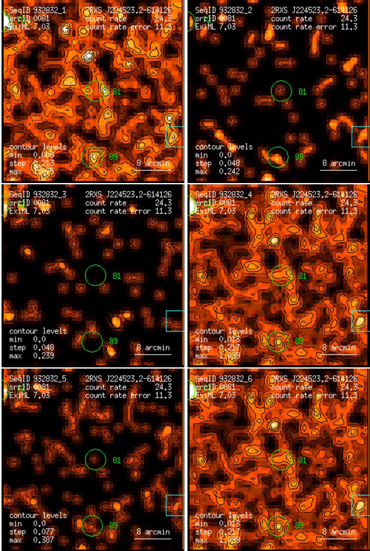
Figure 81: RASS 932832: detection 0081: band rate images, Gaussian filter: (1) PSPC channels 11 – 41, (2) 52 – 90, (3) 91 – 201, (4) 11 – 235, (5) 52 – 201, (6) 11 – 201. Broad band rates in counts/ks. Band rate contour levels in counts/ks/arcmin 2 .
