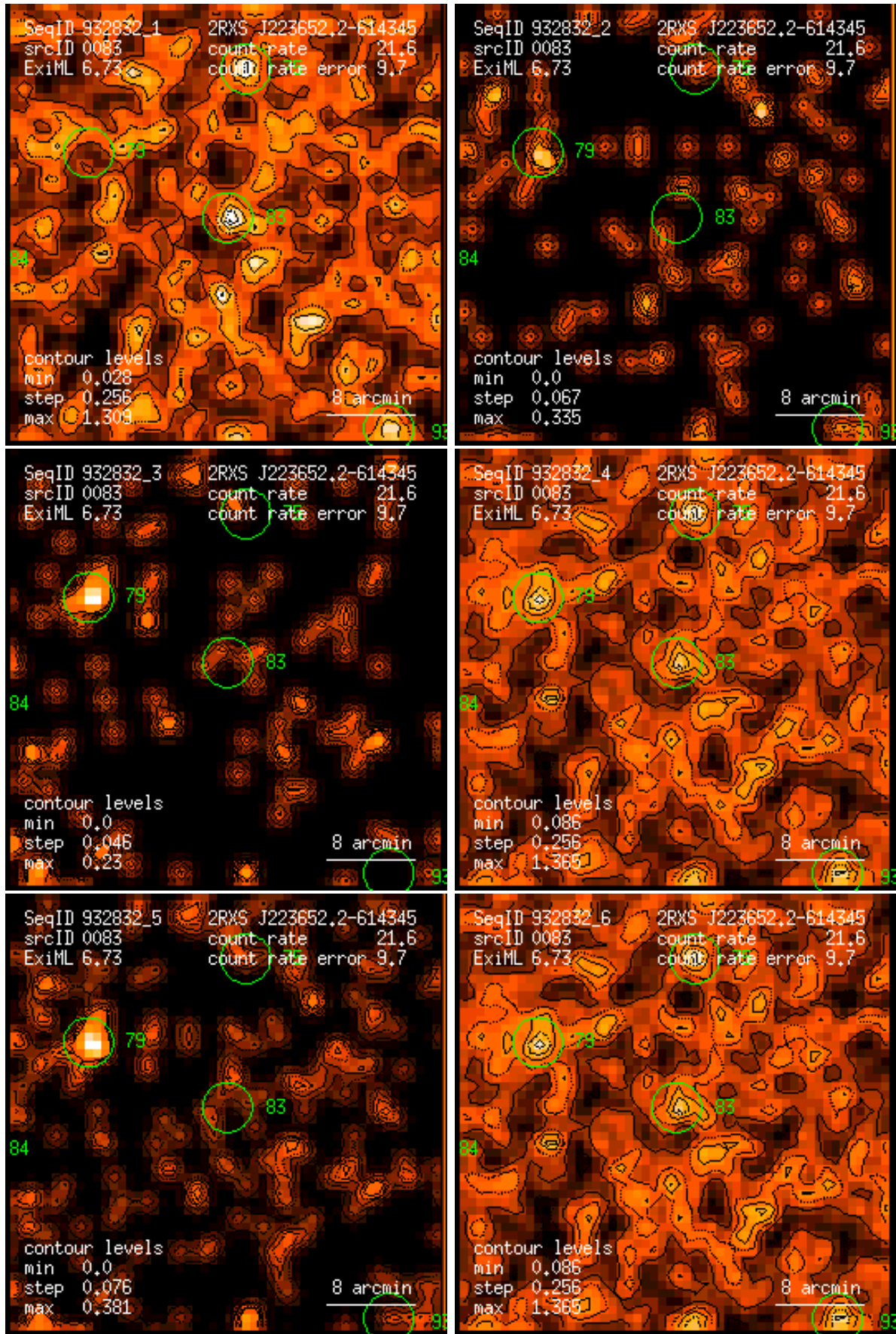
Figure 83: RASS 932832: detection 0083: band rate images, Gaussian filter: (1) PSPC channels 11 – 41, (2) 52 – 90, (3) 91 – 201, (4) 11 – 235, (5) 52 – 201, (6) 11 – 201. Broad band rates in counts/ks. Band rate contour levels in counts/ks/arcmin 2 .
